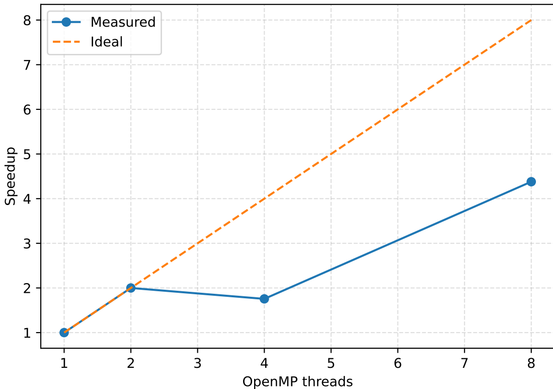
CPU strong scaling (CIC, SoA, unsorted, privatized)
