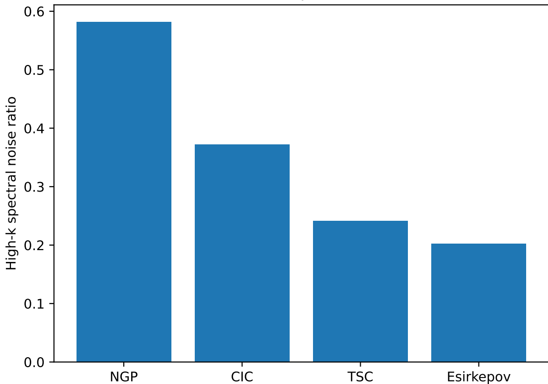
Grid noise vs deposition scheme
