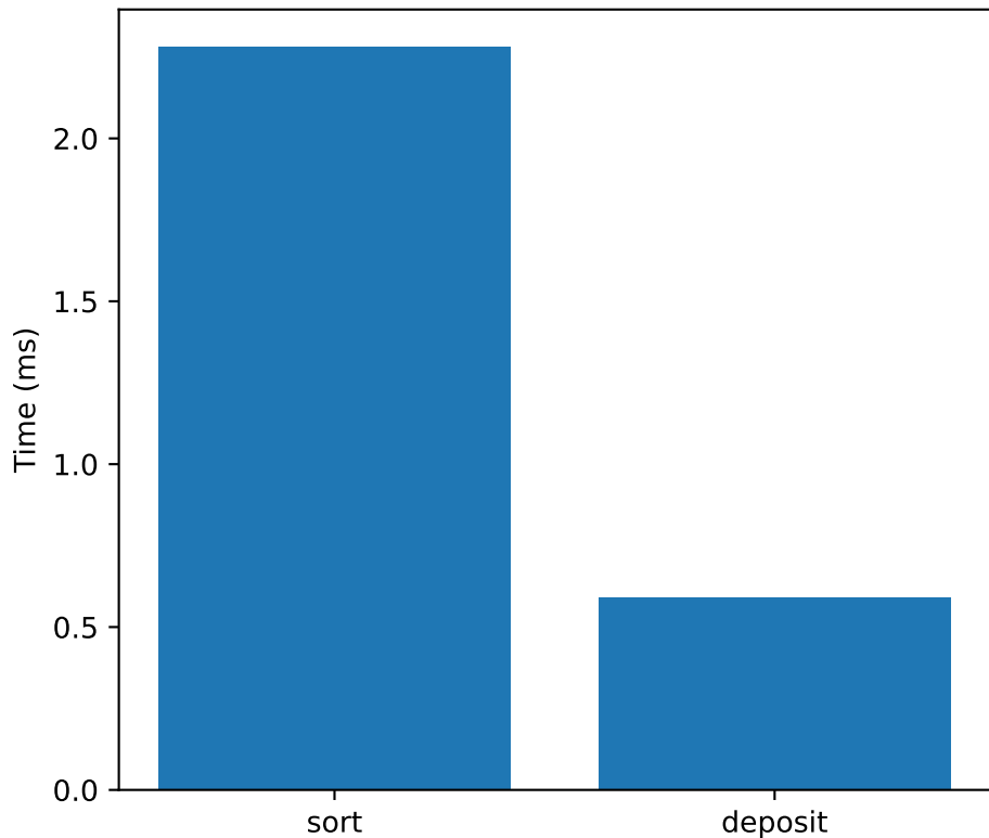
Sort vs deposit cost (CIC, SoA, sorted)
