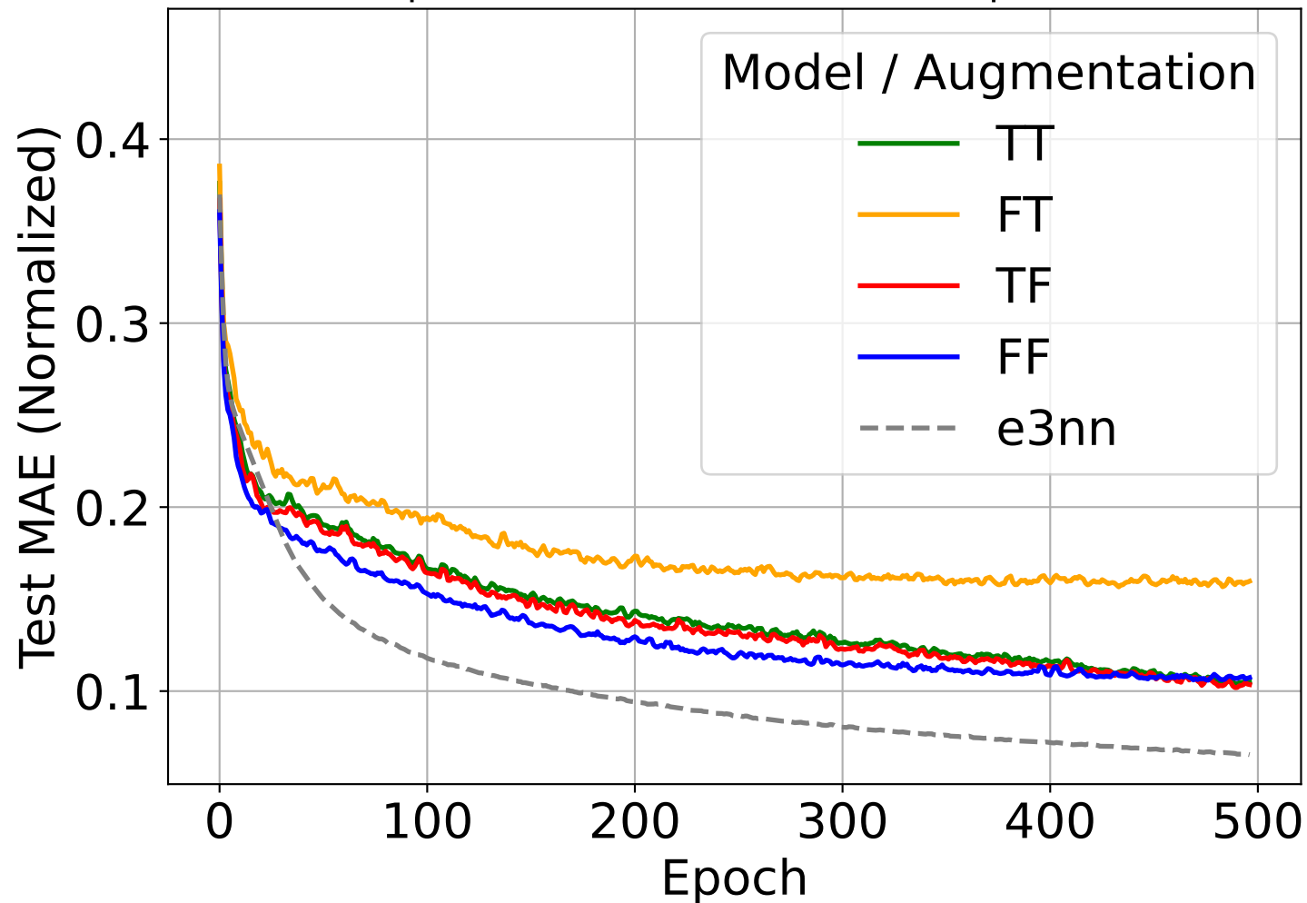
Dipole Moment Test MAE Over Epochs
