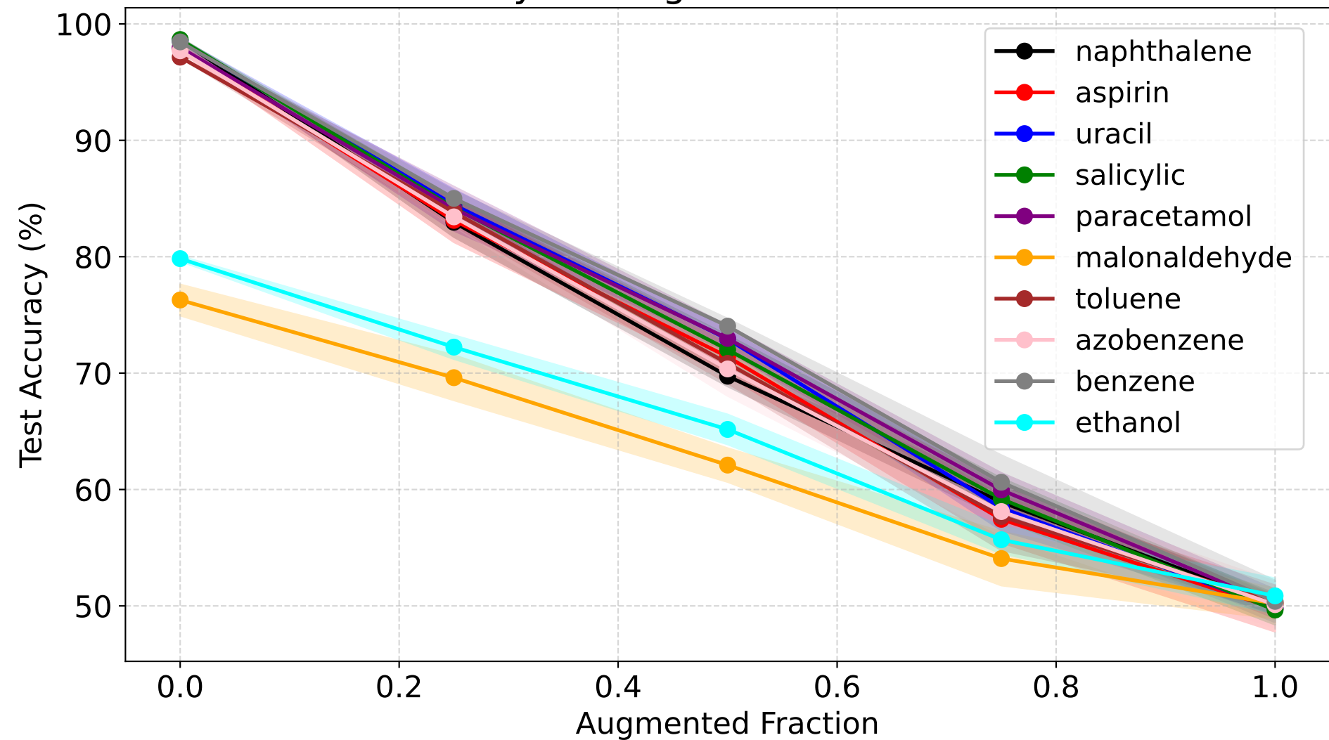
Test Accuracy vs. Augmented Fraction for MD17
