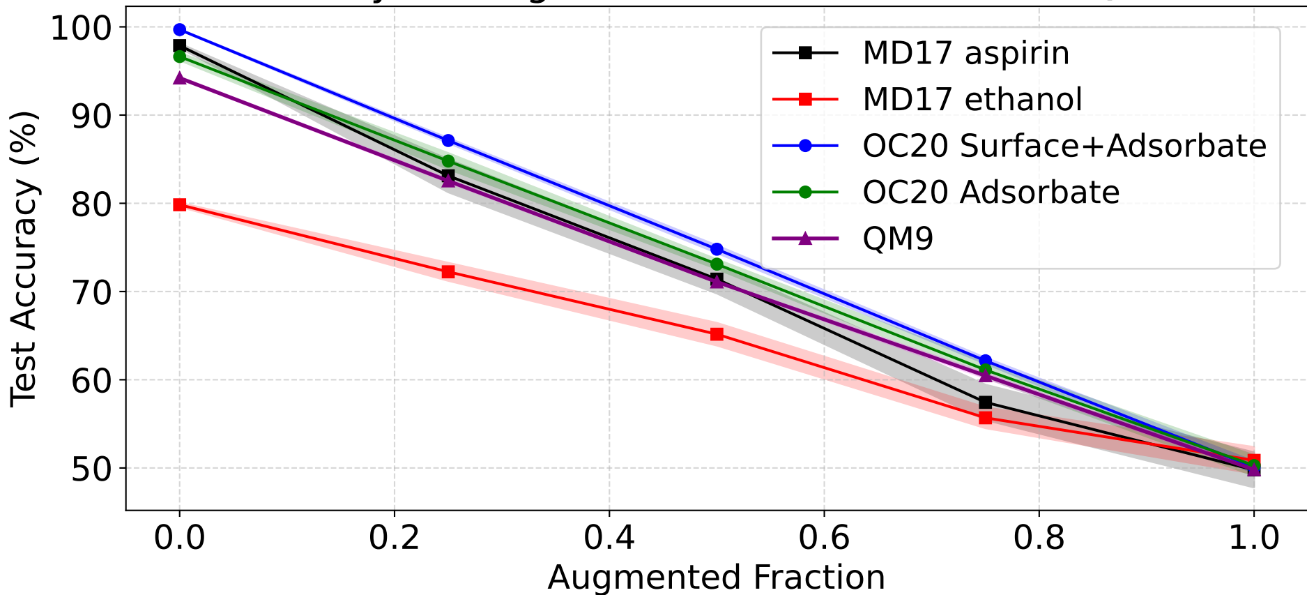
Test Accuracy vs. Augmented Fraction for MD17, QM9, OC20
