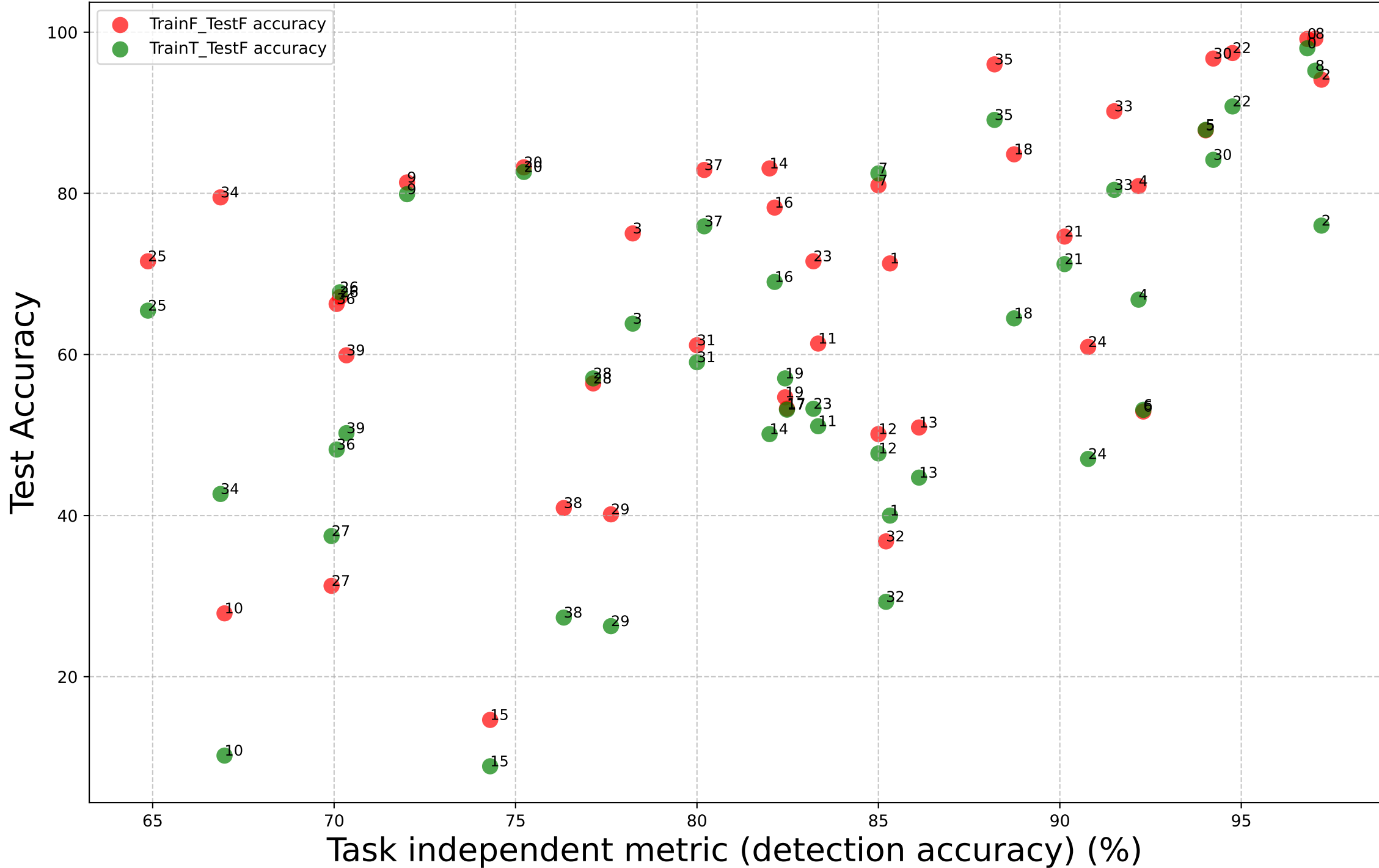
Relation between Task independent metric (detection accuracy) and Test Accuracy on FF/TF settings
