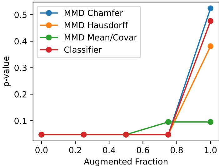
p-value vs Augmented Fraction OC20
