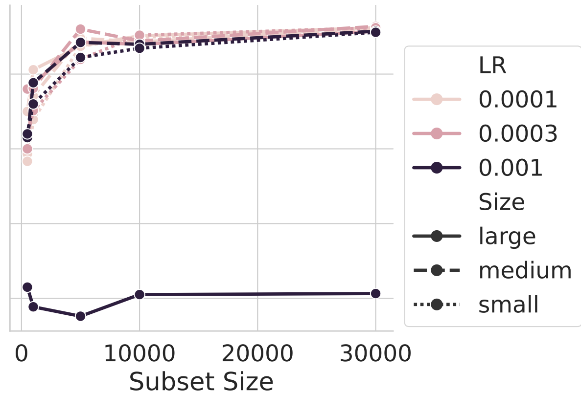
Transformer Architecture
