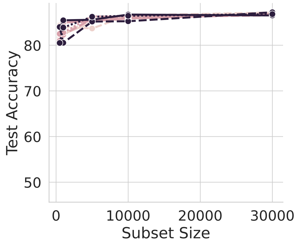
CNN Architecture
