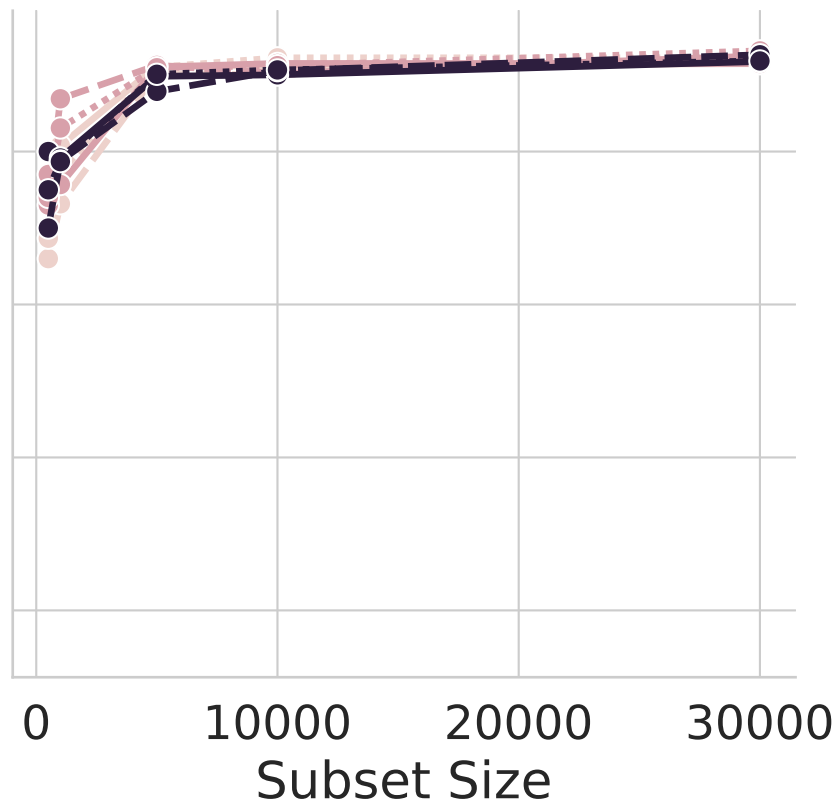
MLP Architecture
