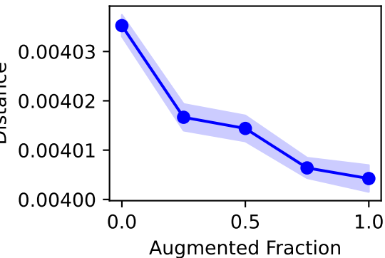
MMD Mean/Covar
