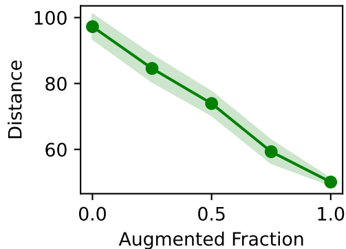
Classifier
