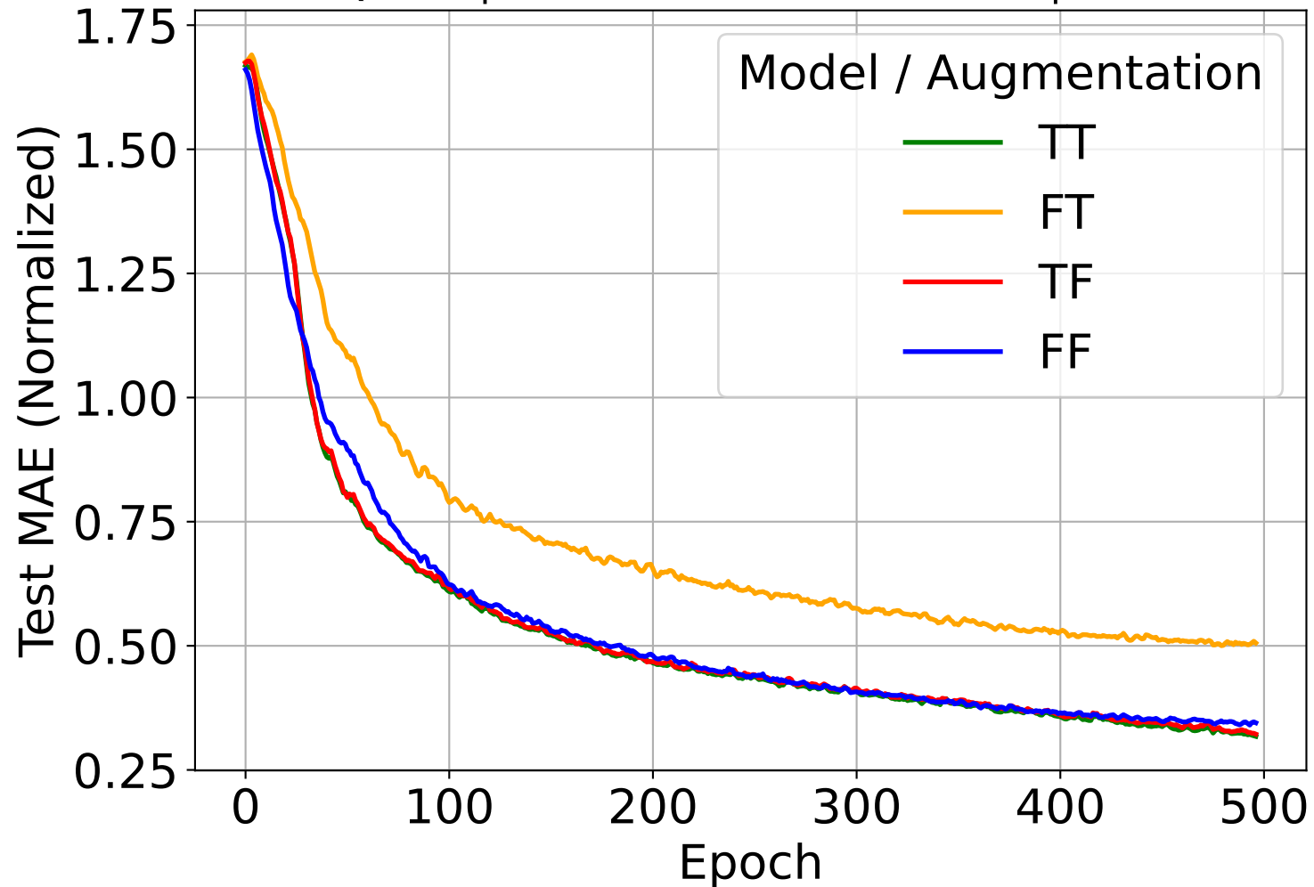
Quadrupole Moment Test MAE Over Epochs
