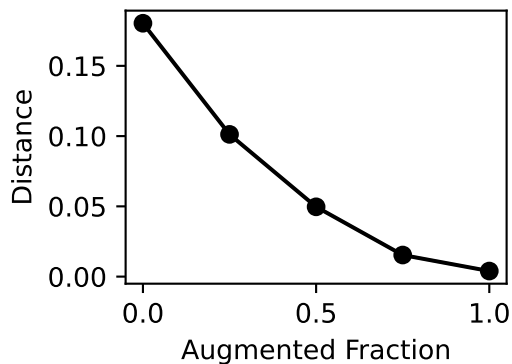
MMD Chamfer
