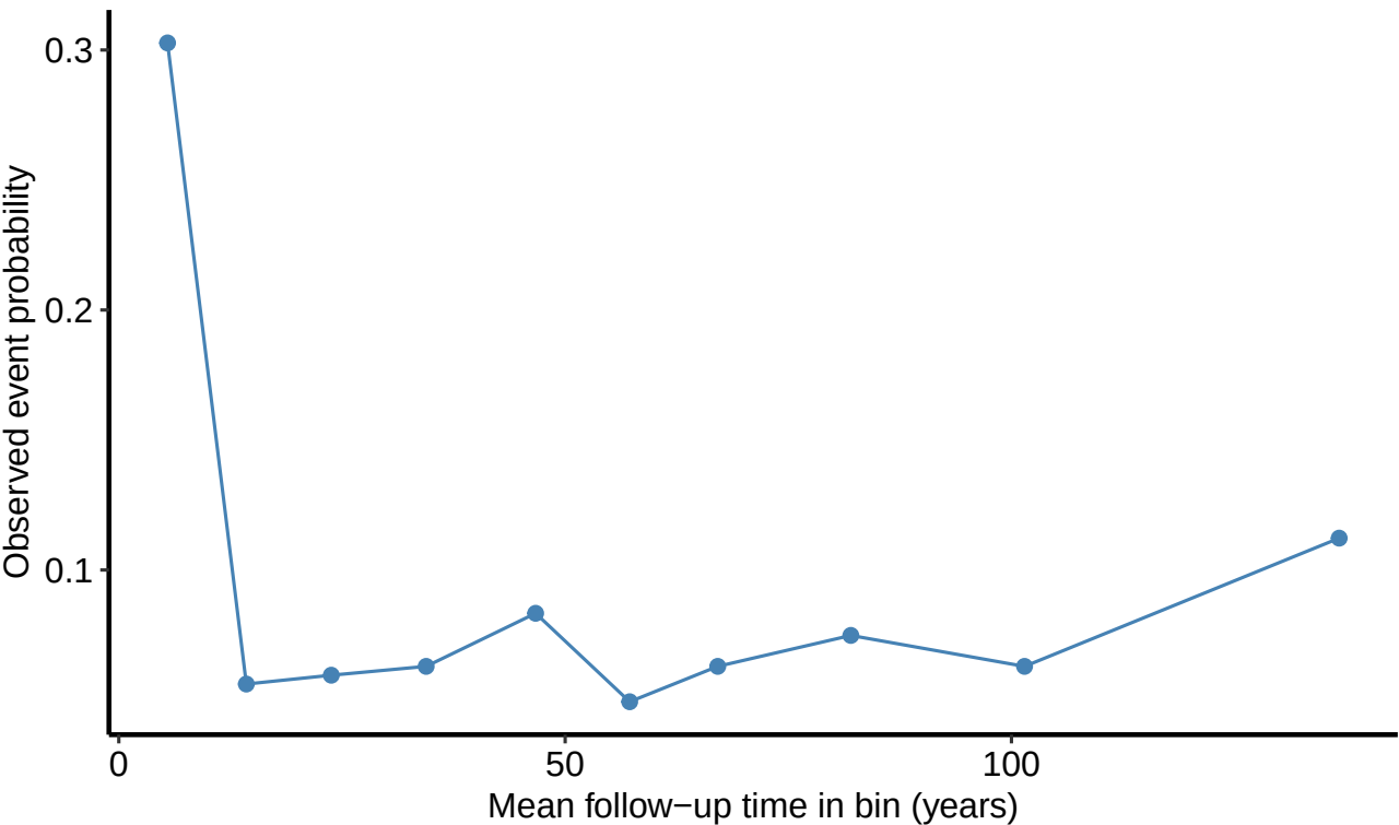
Calibration across follow-up-time deciles
