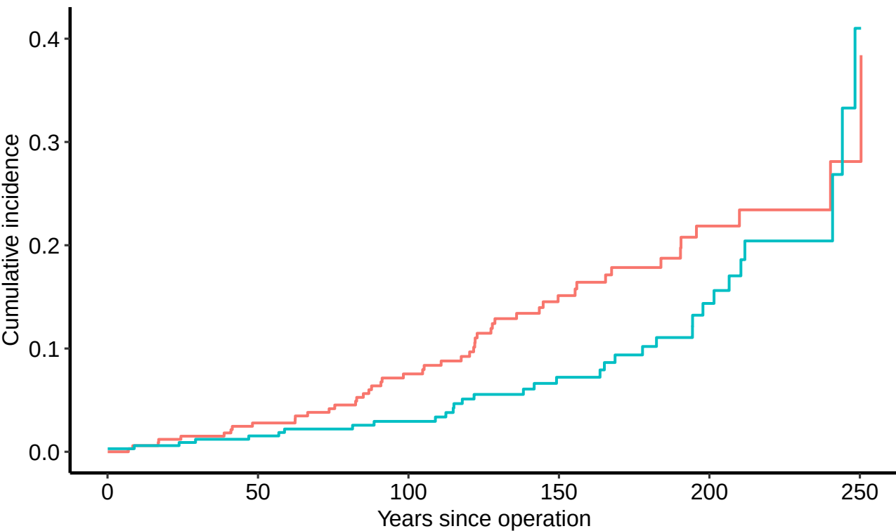
Competing-risks cumulative incidence (omc)
