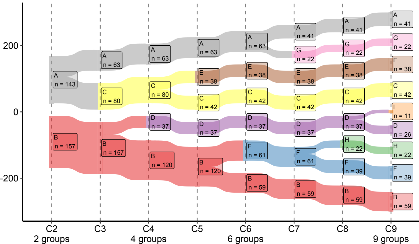
Cluster Stability with group-count milestones
