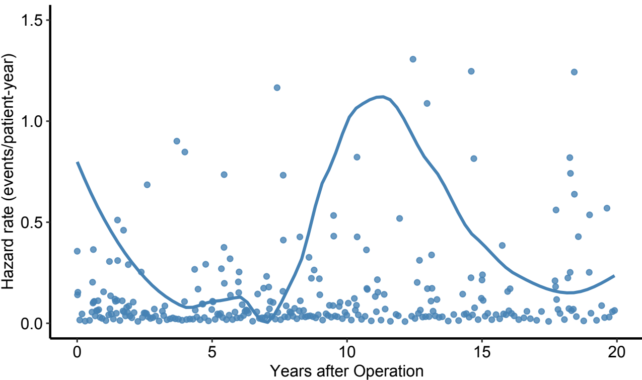
Hazard Rate
