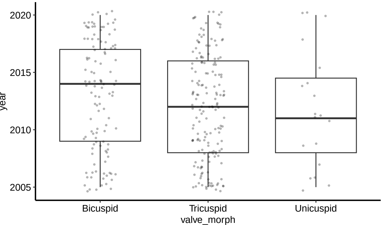
Box plot with jittered observations
