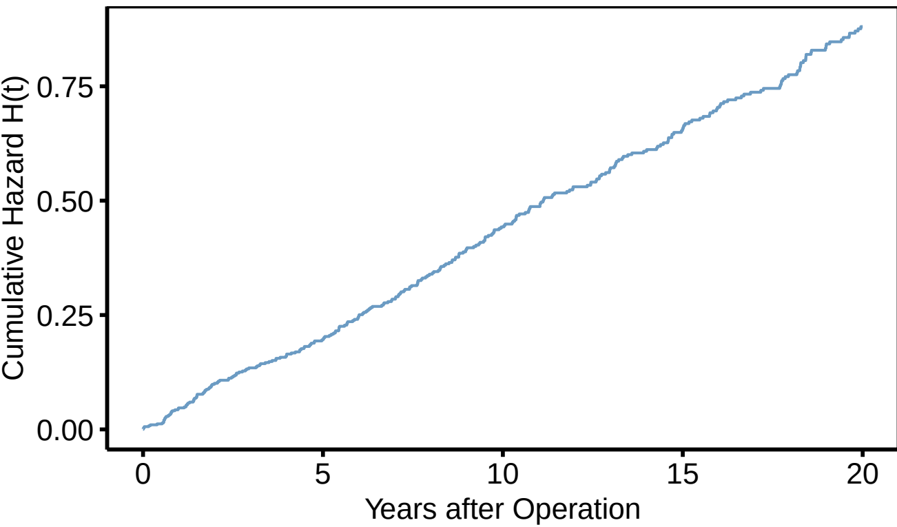
Nelson-Aalen Cumulative Hazard
