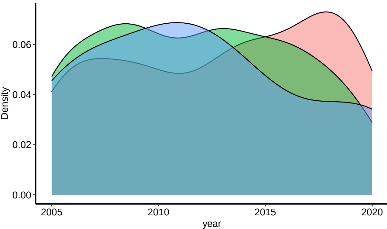
Density by group
