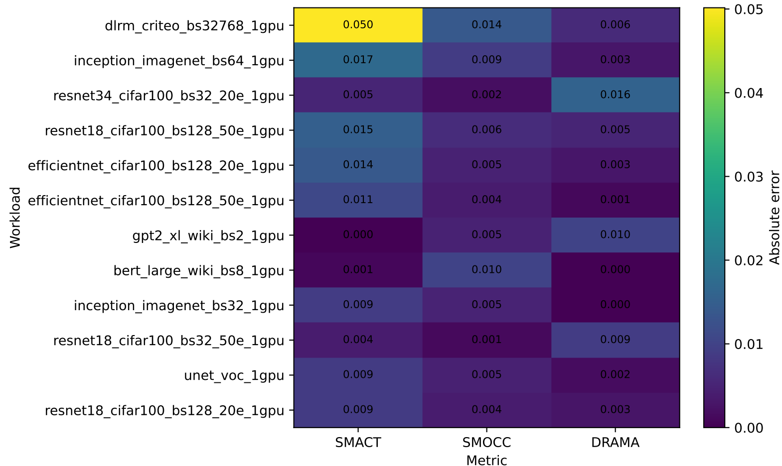
Per-workload P95 error: 40s vs 200s
