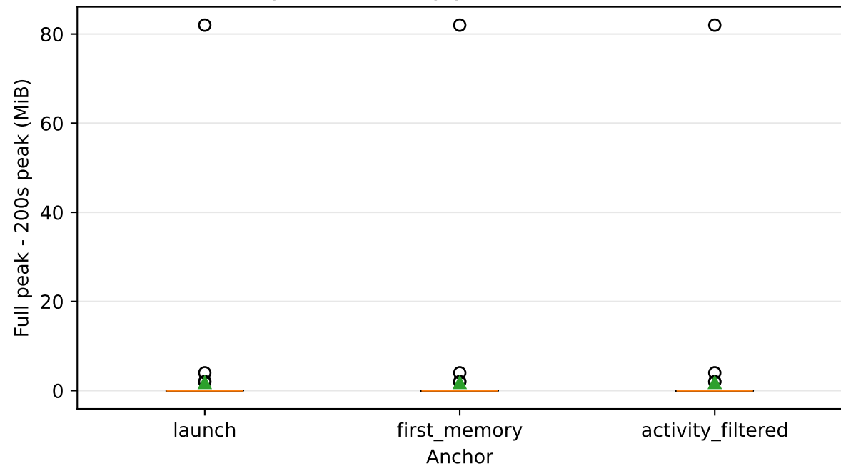
Solo profile memory peak underestimation
