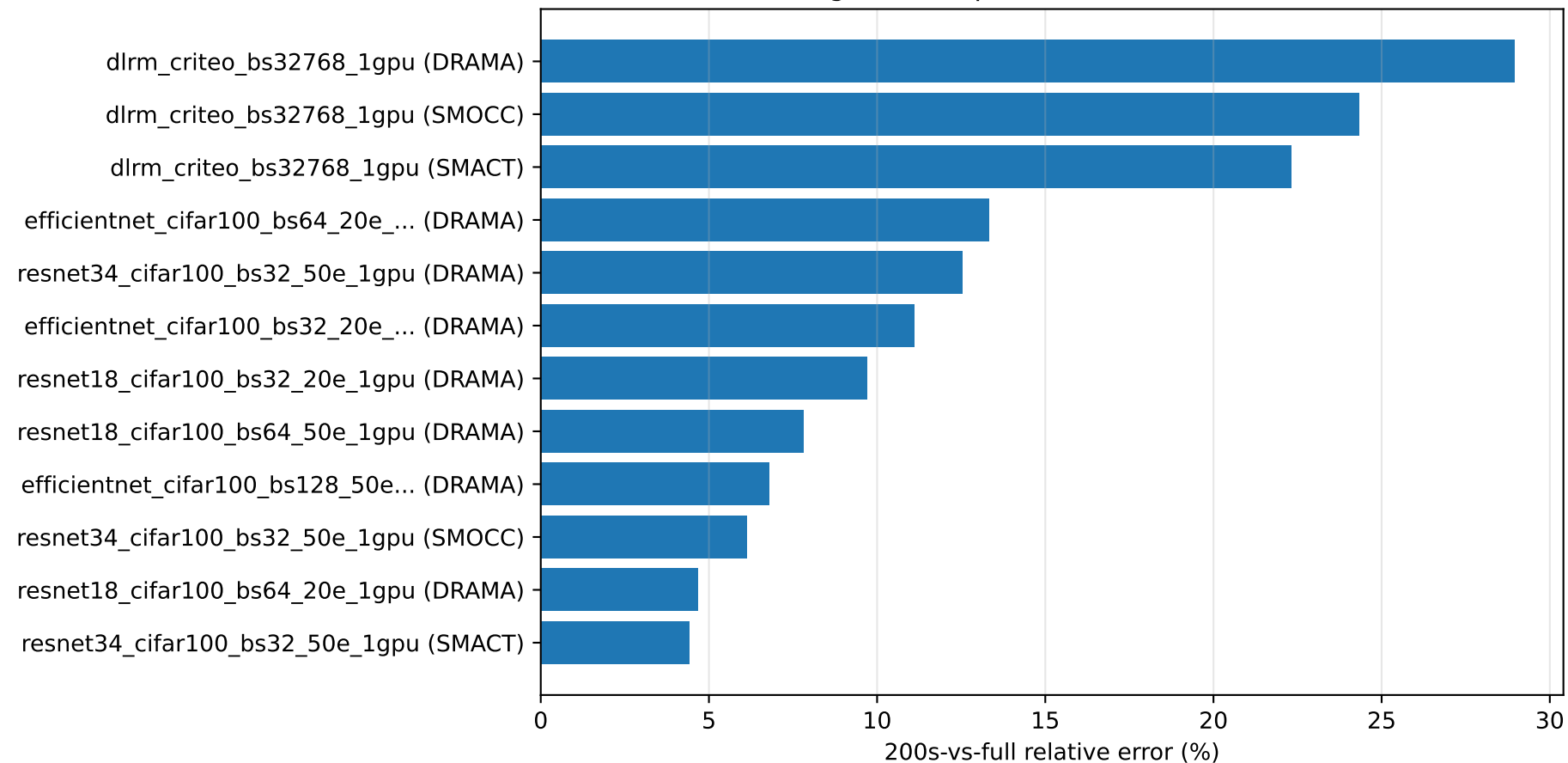
Largest fixed-profile mismatches (P95)
