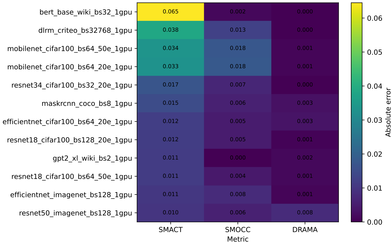
Per-workload MEDIAN error: 60s vs 200s
