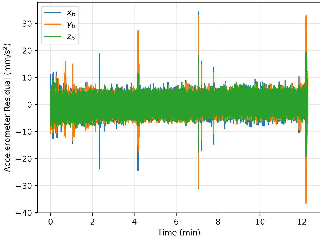
Sensor A Accelerometer Residuals
