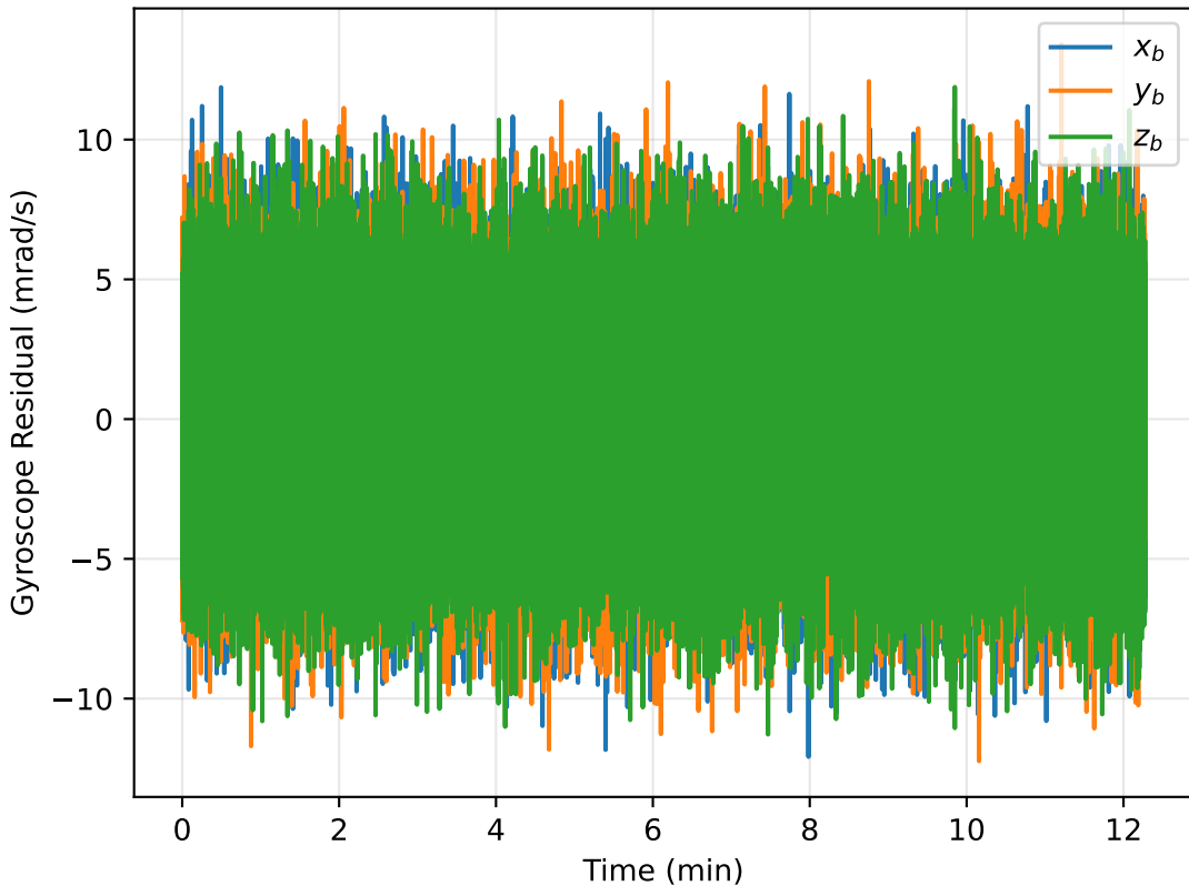
Sensor A Gyroscope Residuals
