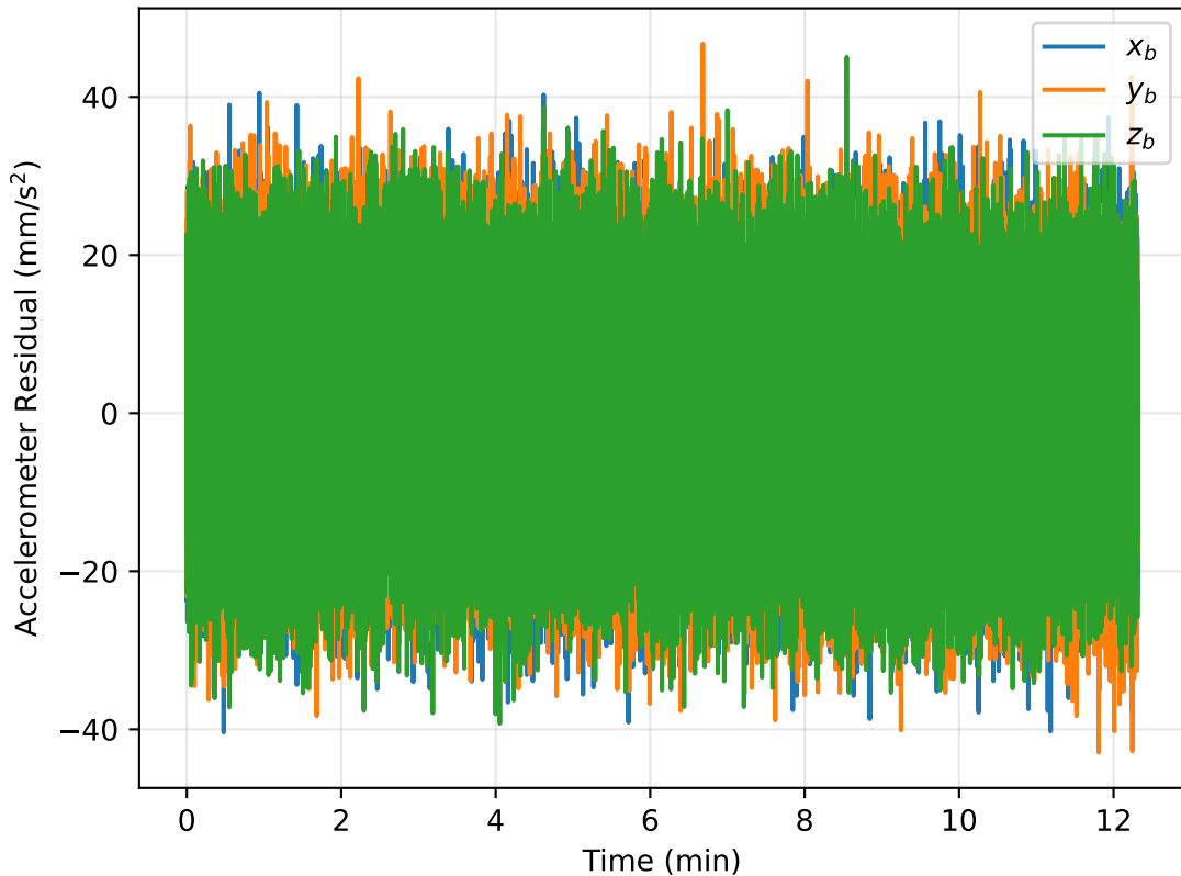
Sensor B Accelerometer Residuals
