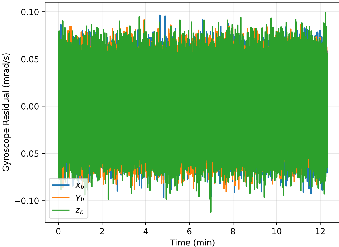
Sensor B Gyroscope Residuals
