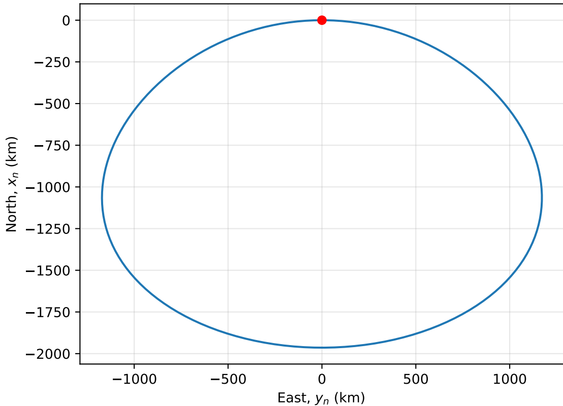
Runway Position Relative to the Aircraft
