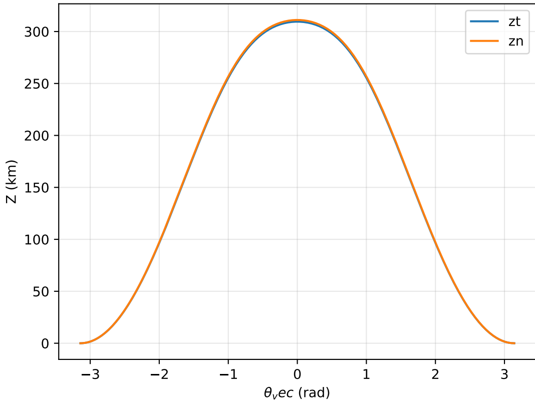
Tangent-Frame Vertical Position vs Navigation-Frame Vertical Position
