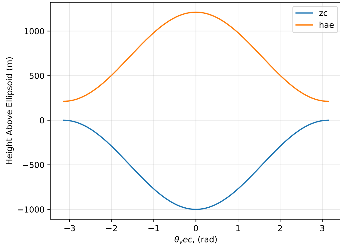
Curvilinear Vertical Coordinate vs Height Above Ellipsoid
