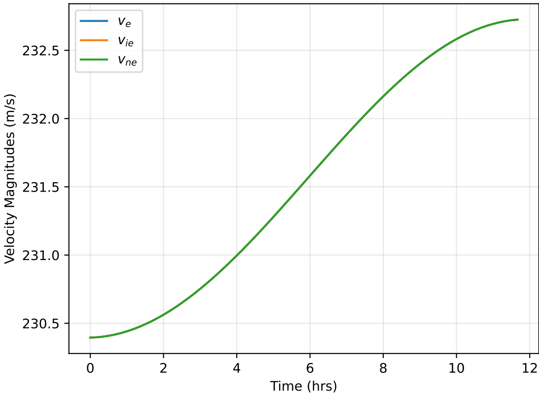
Velocity Magnitude Comparison: Earth-Relative Velocities
