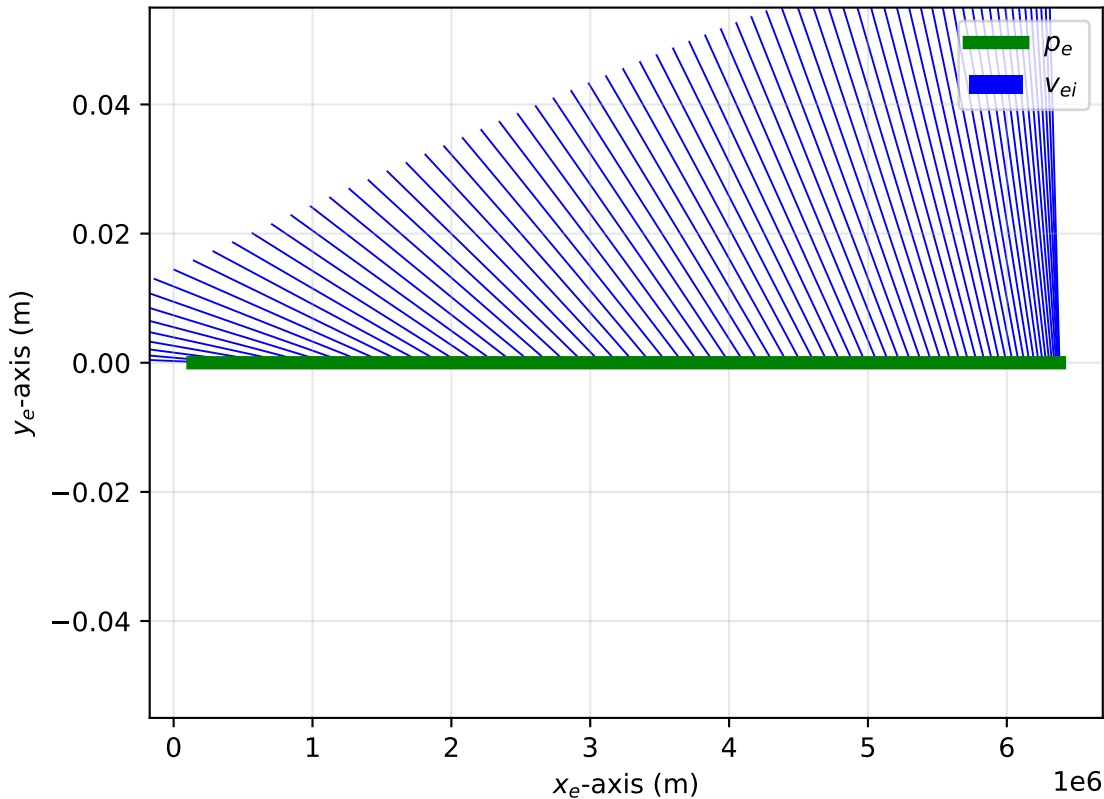
ECEF Position and Inertial-Relative Velocity
