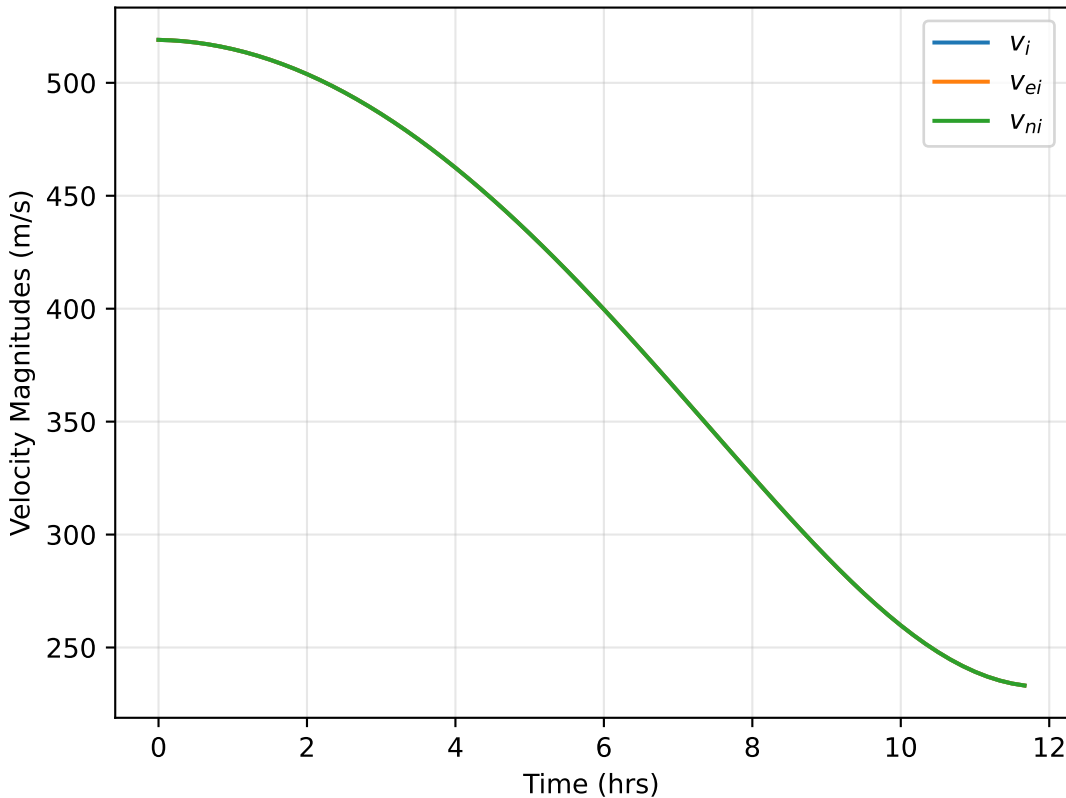
Velocity Magnitude Comparison: Inertial-Relative Velocities
