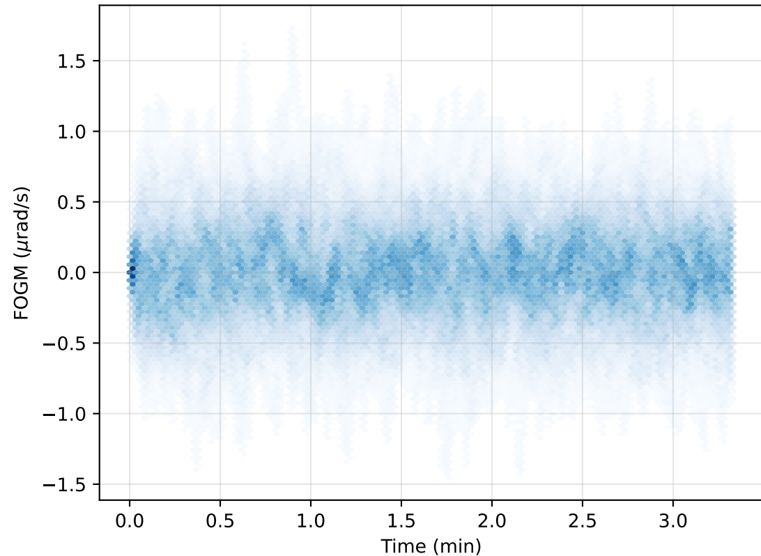
Bias Instability (FOGM) Noise
