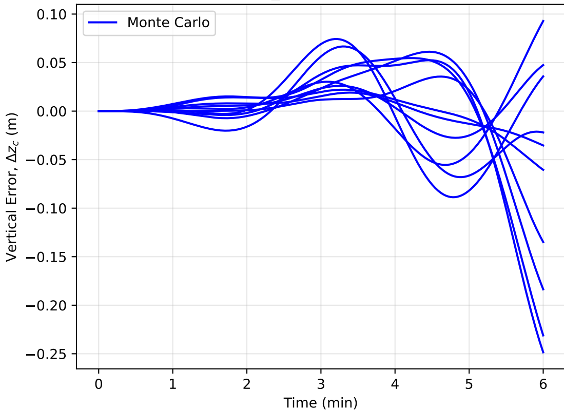
gyro_x: Vertical Error
