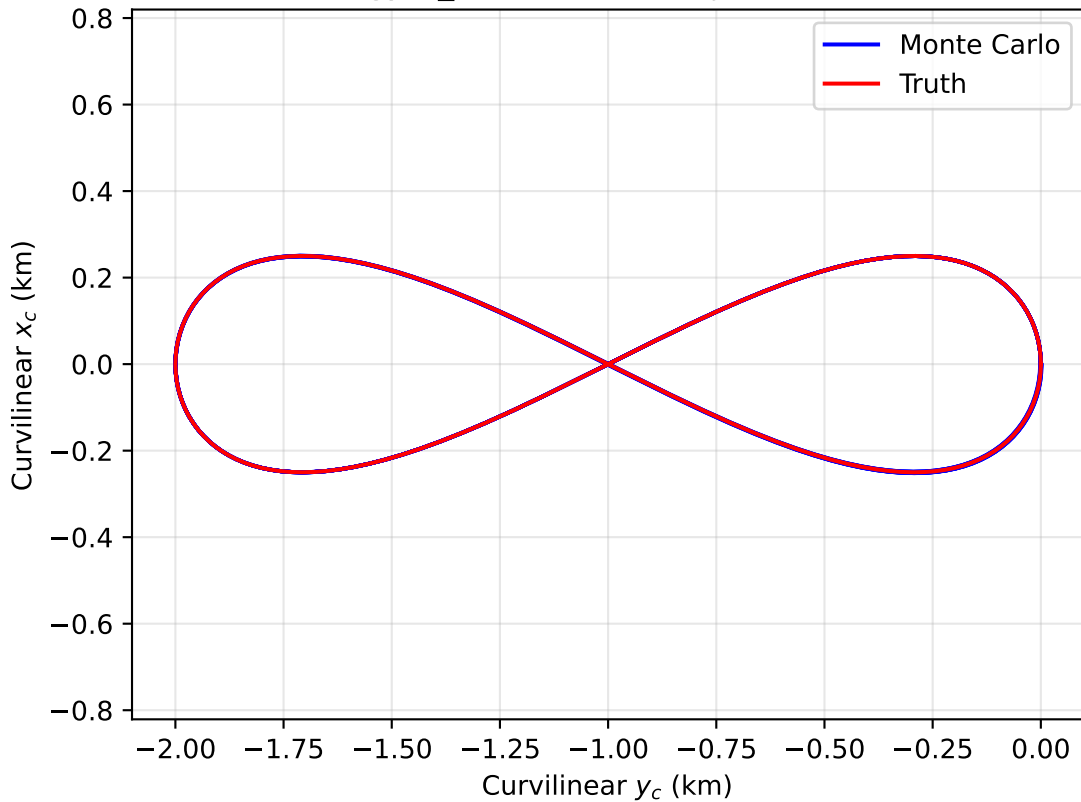
gyro_z: Horizontal Trajectories
