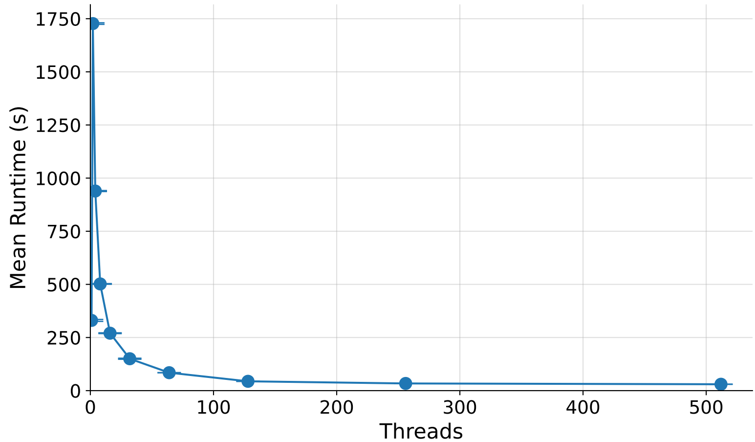
Runtime vs. Thread Count
