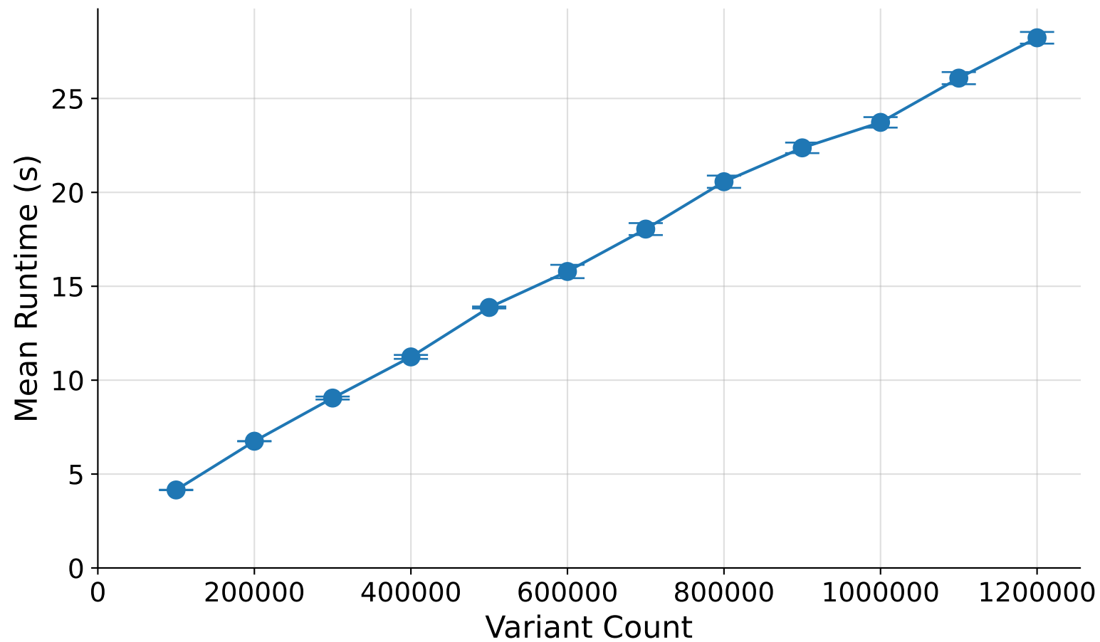
Runtime vs. Variant Count
