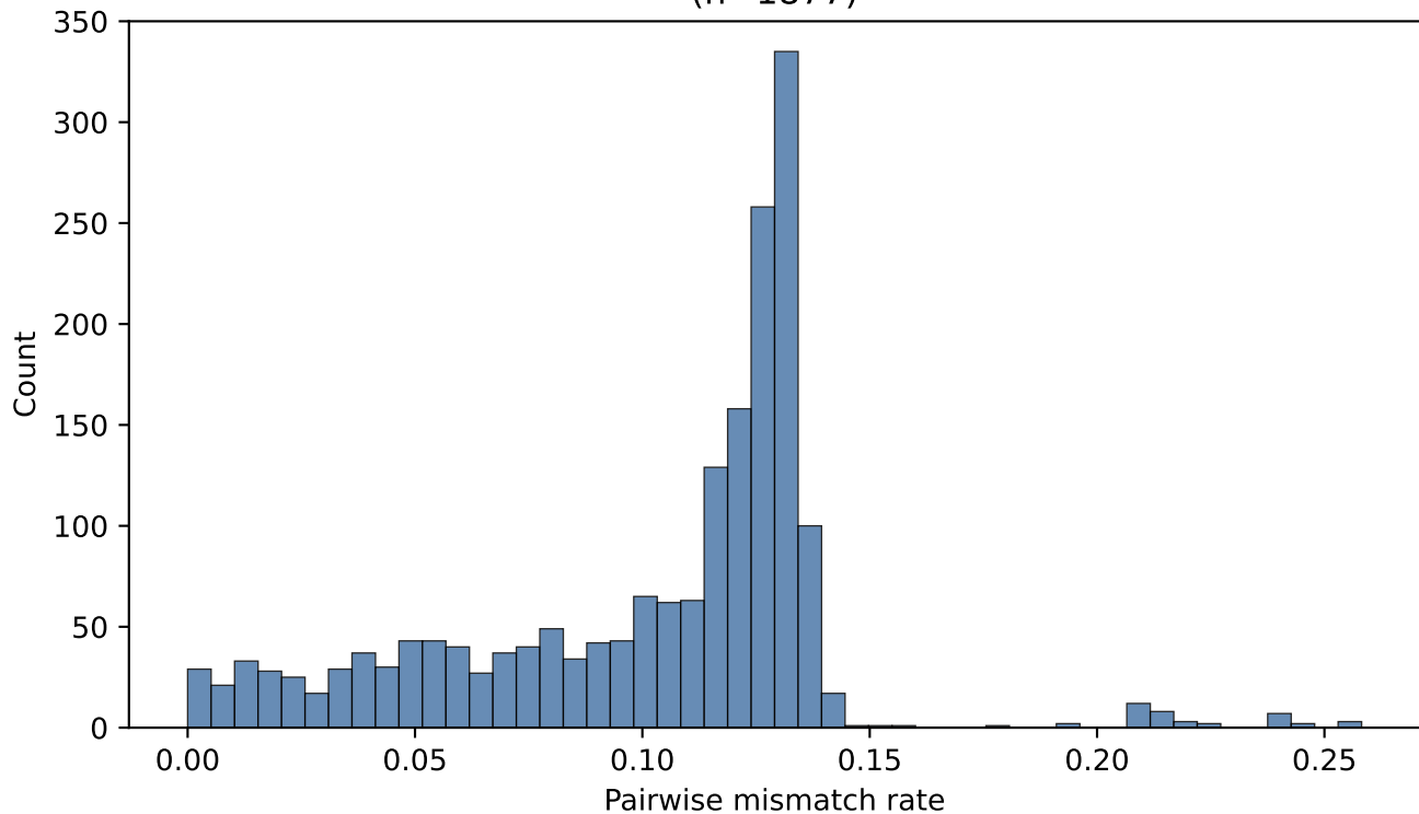
AADR Sample Pairs, Matching Individual IDs (n=1877)
