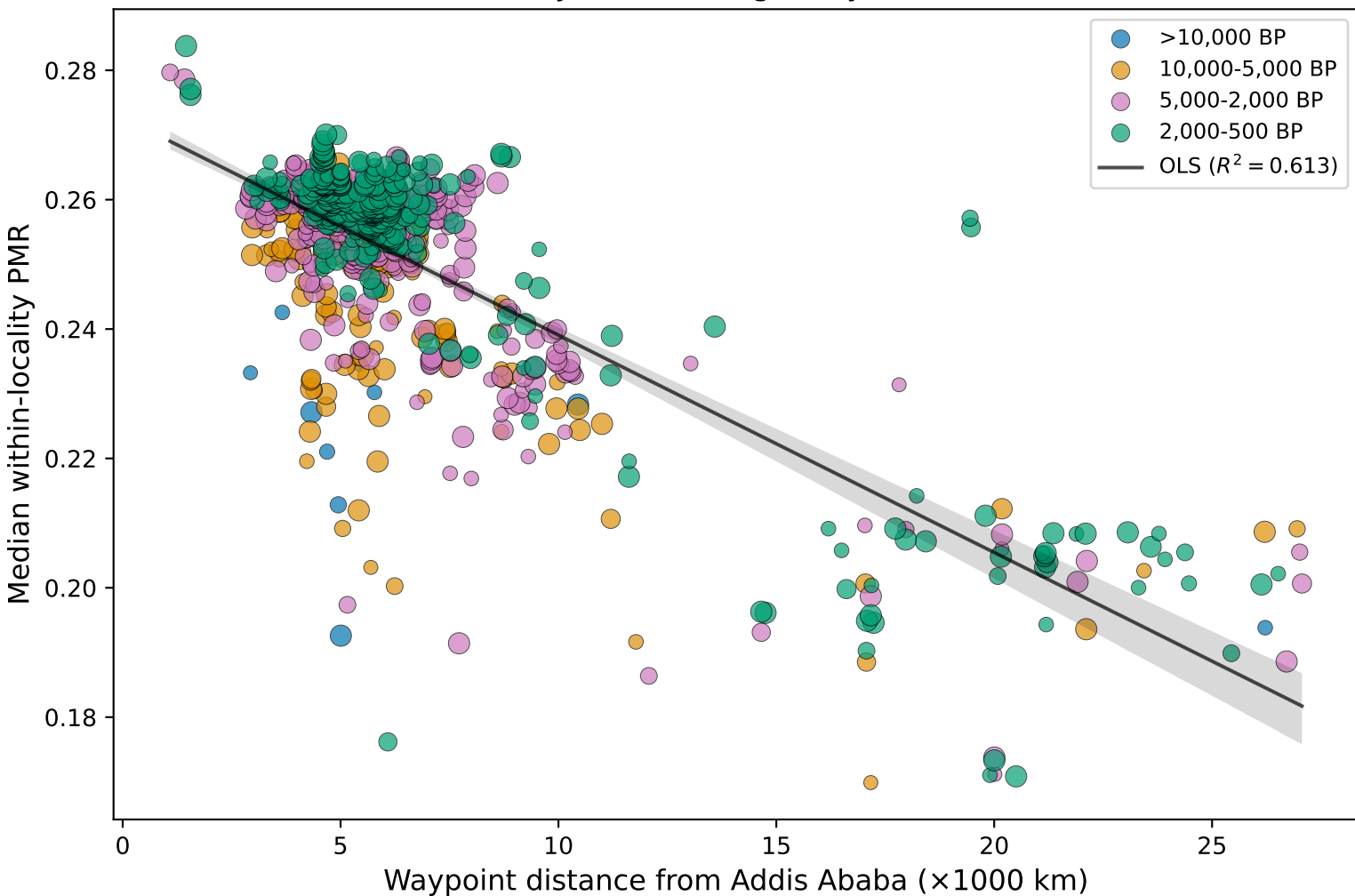
Median within-locality PMR vs. migratory "Out of Africa" distance
