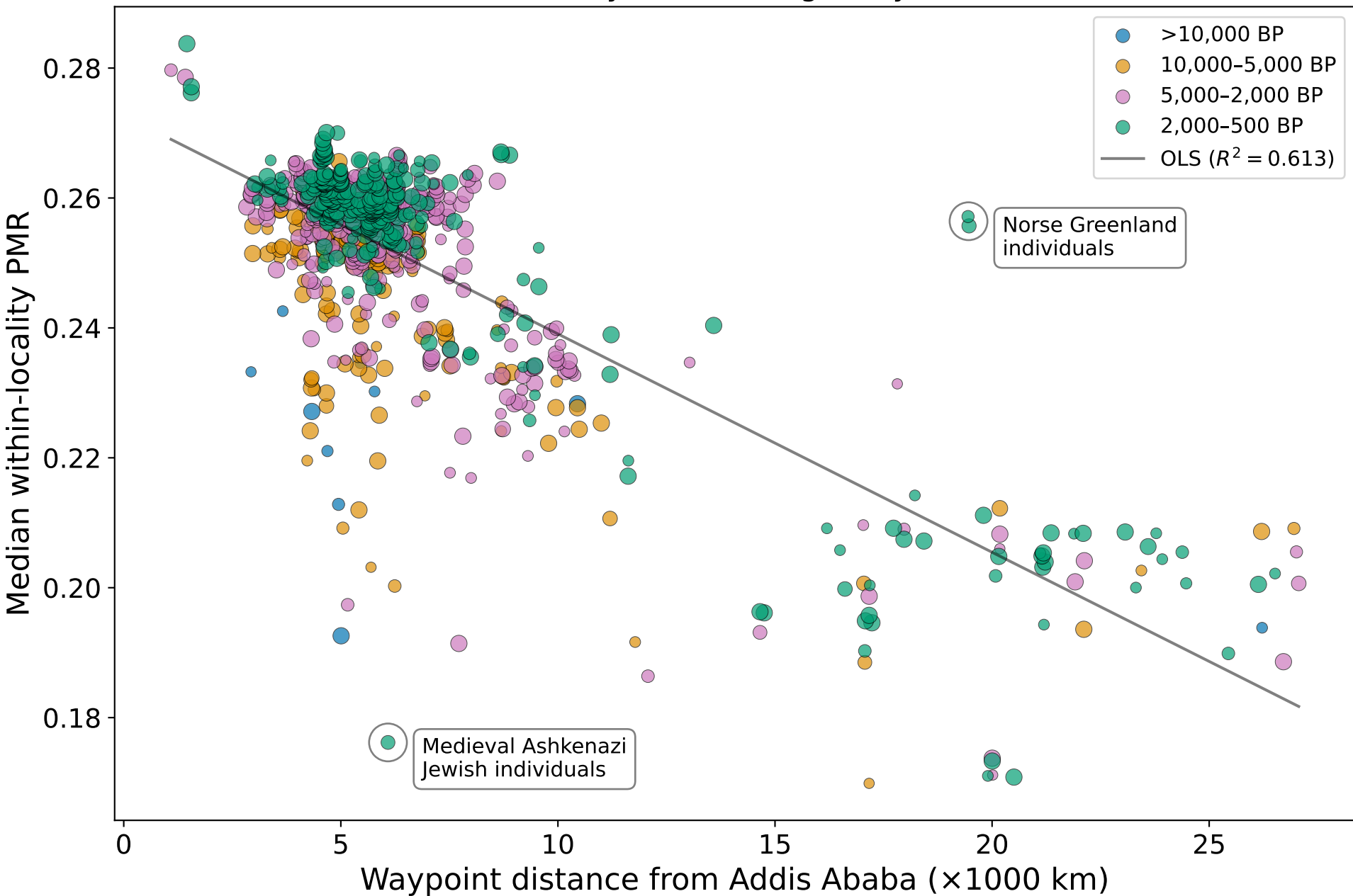
AADR median within-locality PMR vs. migratory "Out of Africa" distance
