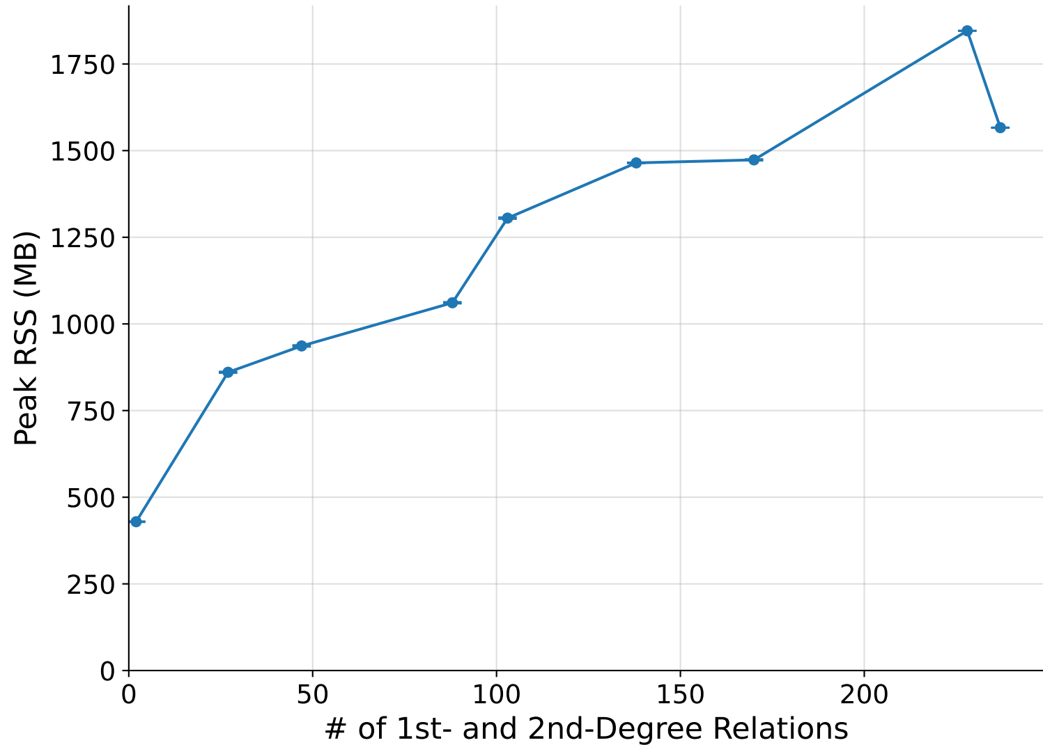
Peak Resident Set Size (RSS) vs. Relations
