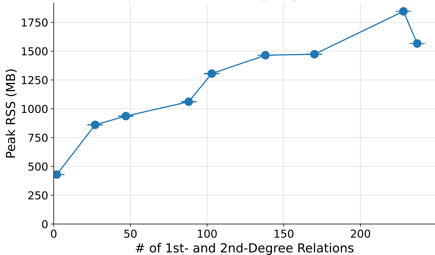
Peak Resident Set Size (RSS) vs. Relations
