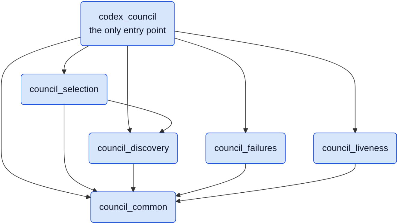
d11-modules — Module responsibilities and imports, verified from the import statements. Source: d11-modules.mmd .
