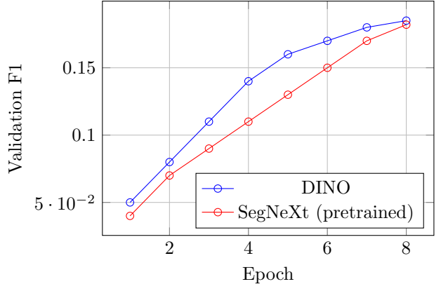
Figure 1. Training dynamics comparison between the DINO baseline and the pretrained SegNeXt-family model.
