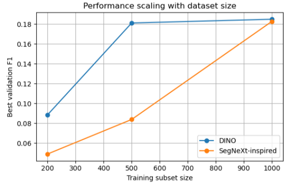
Figure 1. Performance scaling with dataset size for the DINO baseline and the best SegNeXt-family model at each dataset scale. The DINO baseline performs better at smaller dataset sizes, while the pretrained SegNeXt-family variant approaches the DINO result at the largest setting, indicating that representation quality is the key limiting factor.
