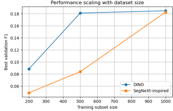
Figure 3. Validation F1 versus dataset size. The DINO baseline performs better at small dataset sizes, while the pretrained SegNeXt-family variant approaches it at the largest setting.
