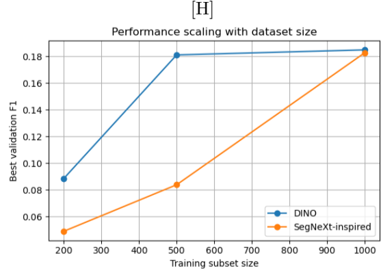
Figure 1. Performance scaling with dataset size for the DINO baseline and the SegNeXt-inspired model. The DINO baseline shows strong performance even at smaller dataset sizes, while the SegNeXt-inspired model benefits more significantly from increased data. At the largest dataset size, the pretrained SegNeXt variant approaches the performance of the DINO baseline, indicating that representation quality is the key limiting factor.
