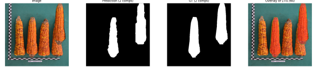
Figure 5. An example from the Kaggle dataset featuring similarities to the MC COCO-generated test set used in Li et al. [9], where our architecture achieves good performance. Note that this is the same image as in figure 1, but with post-processing applied to the predicted mask.
