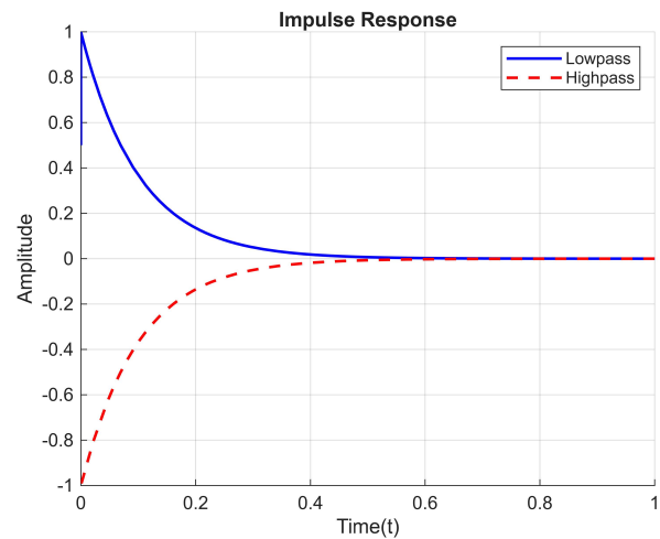
Figure 4. Overlay of filter impulse responses demonstrating complementary decay behaviors.
