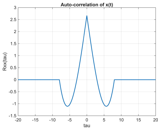
Figure 5. Auto-correlation function highlighting temporal symmetry and peak energy at zero lag.
