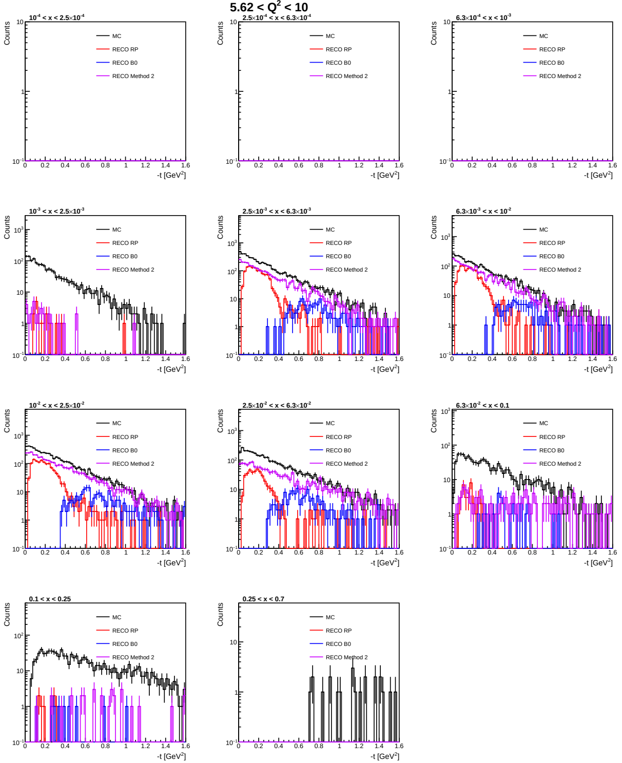
Figure 34: Comparison of the reconstructed -t distributions obtained using the Roman Pot (RP), B0, and Method 2 with the corresponding MC truth distribution for 5.62 < Q^2 < 10 GeV 2 . Each panel represents a different Bjorken- x interval, illustrating the complementary detector acceptance and the contribution of Method 2 in recovering events within regions of reduced RP and B0 acceptance.
