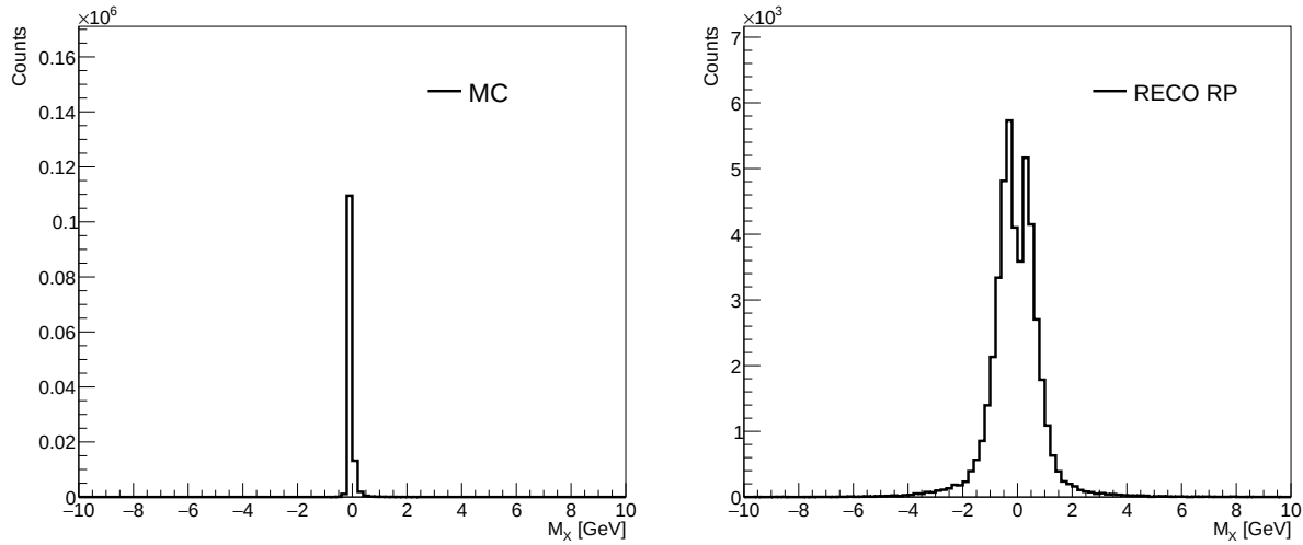
Figure 16: Typical M_X using 26.4.1 10 \times 130 lAger sample; Left - MC, Right - reconstructed RP.
