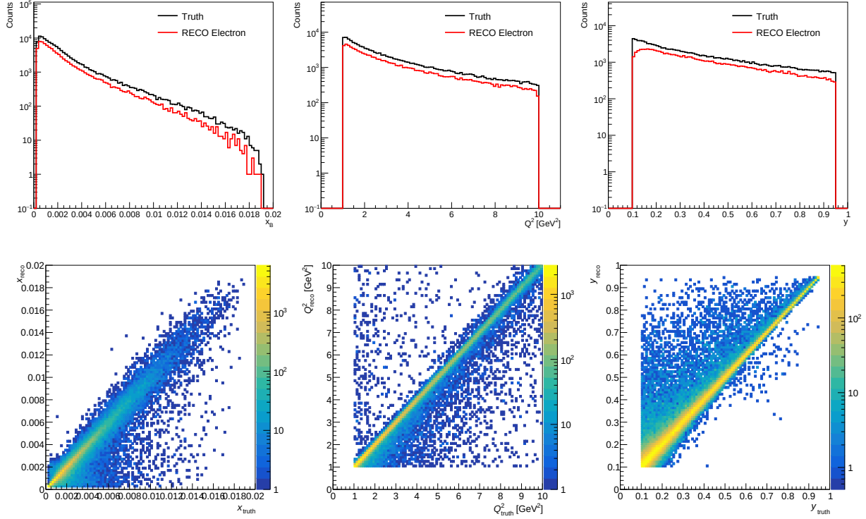
Figure 10: Electron-vertex kinematic variables reconstructed with the Electron Method. From left to right: x , Q^2 , and y . Top row: MC truth and RECO. Bottom row: MC-truth versus RECO correlations.
