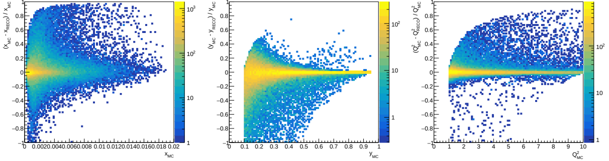
Figure 27: Relative reconstruction resolution for the kinematic variables x_{bj} , y , and Q^2 using the Electron method. Each panel shows the fractional difference (X_{\text{true}} - X_{\text{reco}})/X_{\text{true}} as a function of the true value of the corresponding variable, after applying all quality selections. The distributions illustrate the resolution and possible biases of the electron-based kinematic reconstruction.
