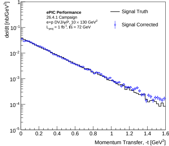
Figure 22: Acceptance-corrected differential cross section obtained after enabling event fallback between the RP, B0, and Method 2 reconstruction regions. Events that cannot be reconstructed using the preferred detector are recovered using an alternative reconstruction method, resulting in a smoother -t spectrum across the detector transition regions. The corrected signal remains in excellent agreement with the generated MC truth over the full momentum-transfer range.
