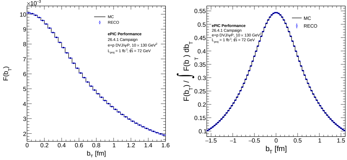
Figure 24: Fourier transform of the differential cross section, providing access to the spatial distribution of quarks within the nucleon.
