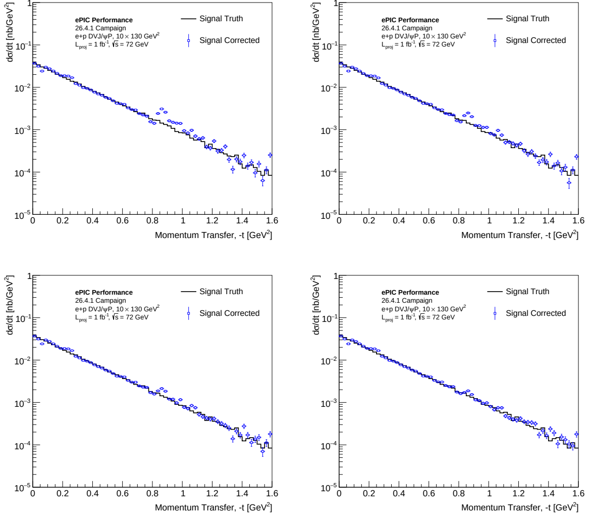
Figure 21: Acceptance-corrected differential cross sections obtained using four different missing-mass: |M_X| < 2 GeV ( top left panel), |M_X| < 5 GeV ( top right panel), |M_X| < 10 GeV ( bottom left panel), and without a missing-mass ( bottom right panel) requirement. Relaxing the missing-mass selection increases the Method 2 statistics in the detector transition region, reducing discontinuities between the RP and B0 reconstruction regions while preserving excellent agreement between the corrected signal and the generated MC truth distribution.
