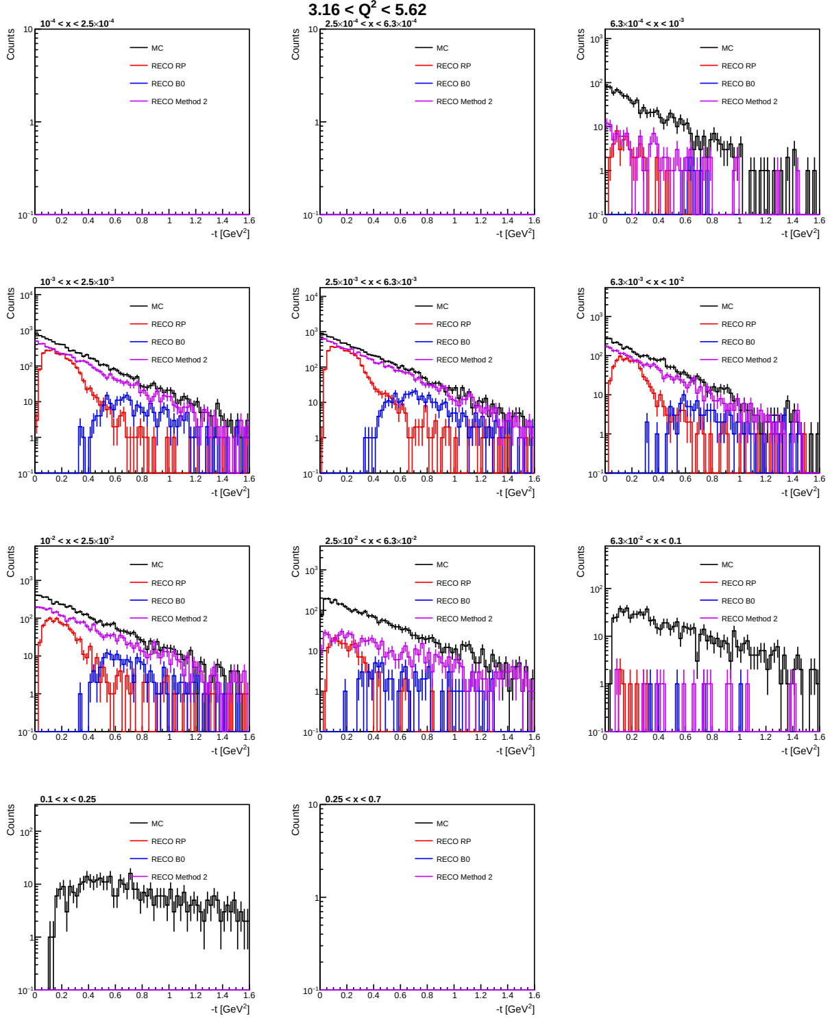
Figure 33: Comparison of the reconstructed -t distributions obtained using the Roman Pot (RP), B0, and Method 2 with the corresponding MC truth distribution for 3.16 < Q^2 < 5.62 \text{ GeV}^2 . Each panel represents a different Bjorken- x interval, illustrating the complementary detector acceptance and the contribution of Method 2 in recovering events within regions of reduced RP and B0 acceptance.
