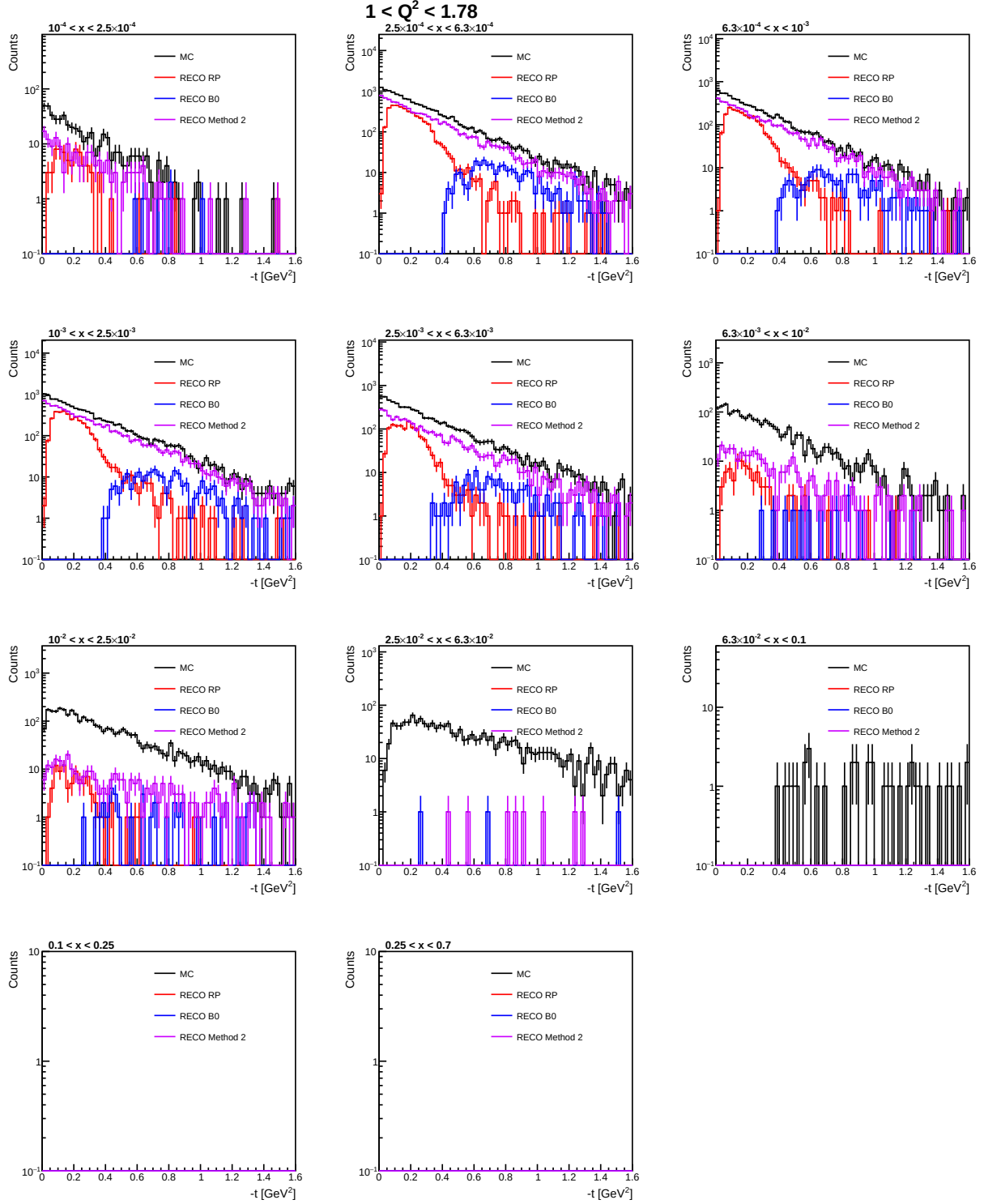
Figure 31: Comparison of the reconstructed -t distributions obtained using the Roman Pot (RP), B0, and Method 2 with the corresponding MC truth distribution for 1 < Q^2 < 1.78 \text{ GeV}^2 . Each panel represents a different Bjorken- x interval, illustrating the complementary detector acceptance and the contribution of Method 2 in recovering events within regions of reduced RP and B0 acceptance.
