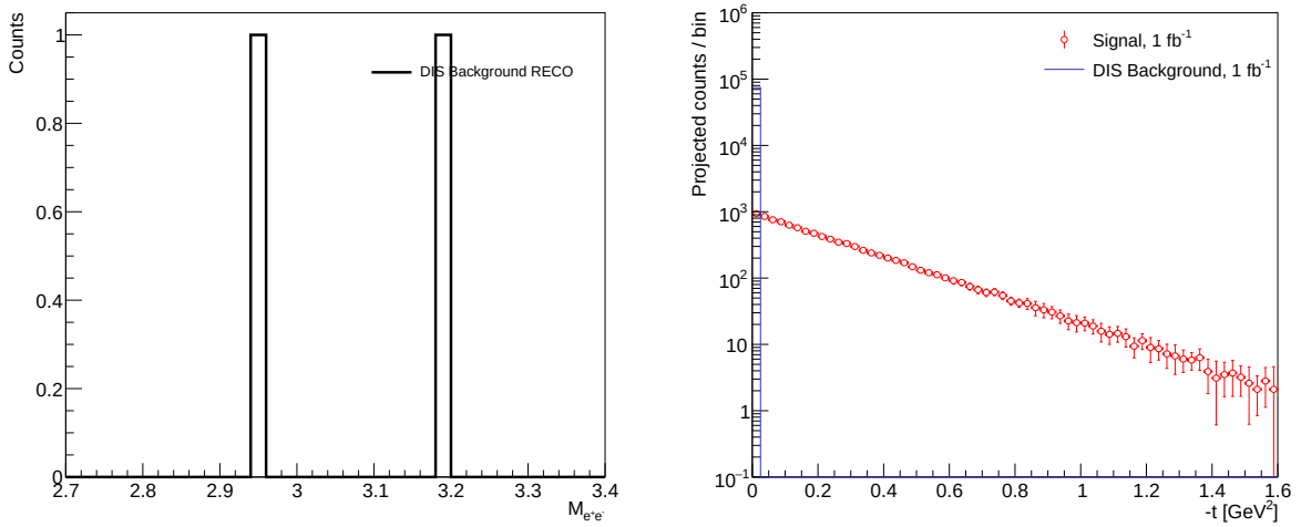
Figure 25: Comparison of reconstructed inclusive DIS background surviving the exclusive J/\psi \rightarrow e^+e^- DVMP analysis selections after applying all quality and exclusivity cuts. The distributions show the reconstructed invariant mass ( Left ) and the projected event yields as a function of -t for an integrated luminosity of 1 \text{ fb}^{-1} . ( Right ), using the kinematic reconstruction methods discussed in Sections 5.2 and 5.3 and discussed in Section 5.4. The signal and DIS background yields are scaled to an integrated luminosity of 1 \text{ fb}^{-1} .
