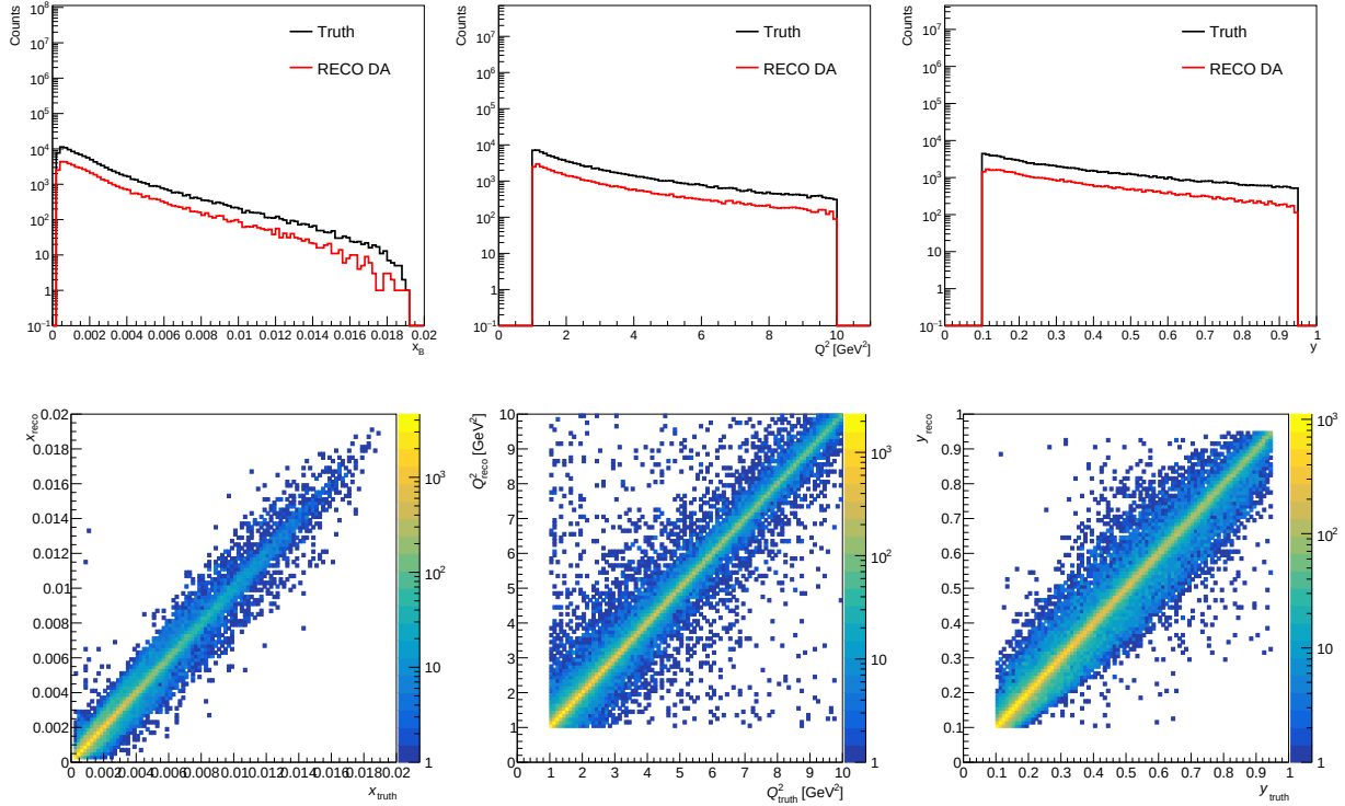
Figure 9: Kinematic variables reconstructed with the DA method. From left to right: x , Q^2 , and y . Top row: MC truth and RECO. Bottom row: MC-truth versus RECO correlations.
