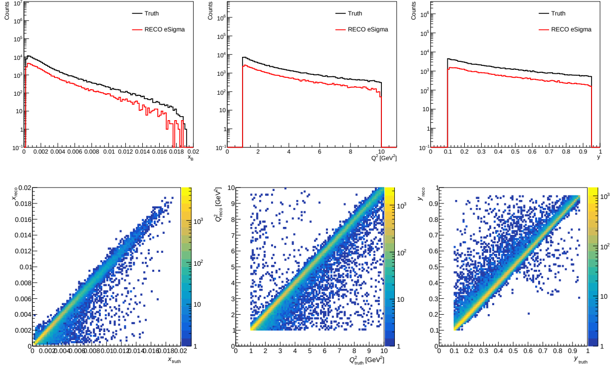
Figure 8: Electron-vertex kinematic variables reconstructed with the e\Sigma method. From left to right: x , Q^2 , and y . Top row: MC truth and RECO. Bottom row: MC-truth versus RECO correlations.
