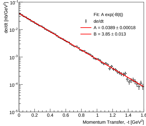
Figure 23: Determination of the t -slope parameter from the differential cross section. The differential cross section is fitted with the exponential function d\sigma/dt = Ae^{-B|t|} , yielding a slope parameter of B = 3.85 \pm 0.013 \text{ GeV}^{-2} . The fitted function provides an excellent description of the simulated -t dependence over the full kinematic range.
