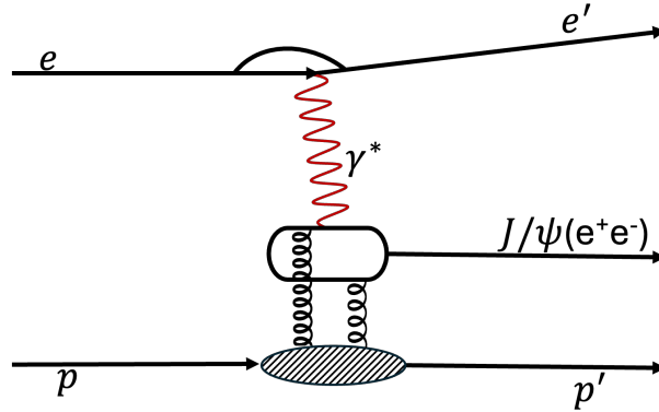
Figure 6: Exclusive process at the EIC illustrating J/\psi production with the e^+e^- decay channel [2], as shown in Eq. 1. This topology requires precise measurements of all final-state particles to ensure event exclusivity. Other J/\psi decay channels are also possible but are not shown here.
