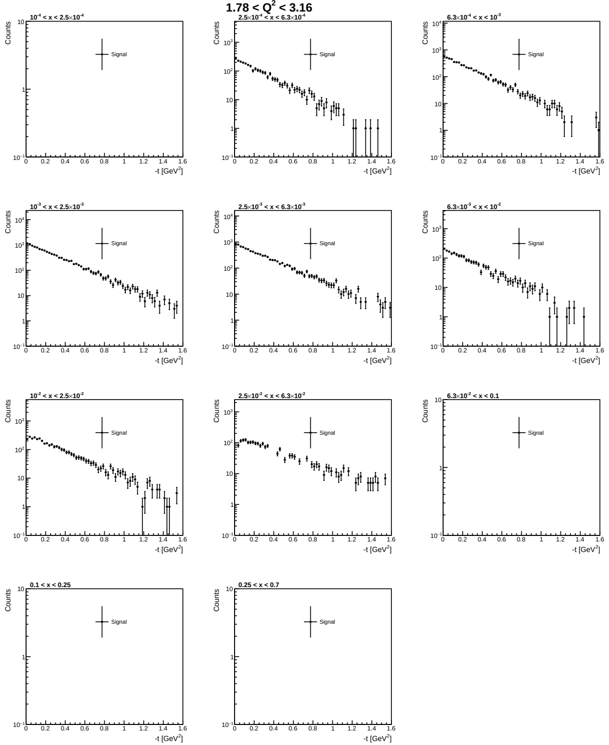
Figure 36: Comparison of the MC truth and acceptance-corrected reconstructed -t distributions for 1.78 < Q^2 < 3.16 GeV 2 . The fallback reconstruction improves the event recovery across the detector transition regions, yielding good agreement between the corrected and generated distributions throughout the populated (Q^2, x) bins.
