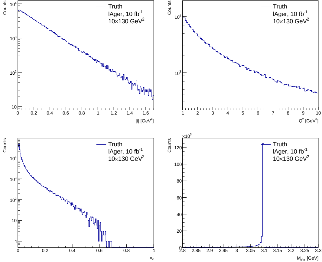
Figure 3: Generator-level kinematic distributions for exclusive J/\psi electroproduction in 10 \times 130 \text{ GeV} ep collisions corresponding to an integrated luminosity of 10 \text{ fb}^{-1} . The panels show ( top left ) the absolute squared four-momentum transfer, |t| , ( top right ) the photon virtuality, Q^2 , ( bottom left ) the Bjorken scaling variable, x_v , and ( bottom right ) the invariant mass of the generated e^+e^- pair. The |t| , Q^2 , and x_v distributions are displayed on logarithmic scales to emphasize the broad kinematic coverage of the generated event sample. The invariant mass distribution exhibits a narrow peak at the nominal J/\psi mass, confirming the correct reconstruction of the generated decay products.
