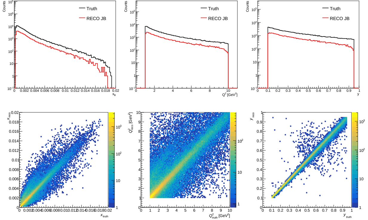
Figure 7: Electron-vertex kinematic variables reconstructed with the JB method. From left to right: x , Q^2 , and y . Top row: MC truth and RECO. Bottom row: MC-truth versus RECO correlations.
