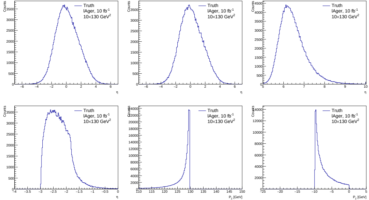
Figure 4: Generator-level pseudorapidity ( \eta ) and longitudinal momentum ( P_z ) distributions for the final-state particles in exclusive J/\psi electroproduction at the ePIC EIC for 10 \times 130 GeV ep collisions corresponding to an integrated luminosity of 10 \text{ fb}^{-1} . The top row shows the pseudorapidity distributions of the J/\psi decay electron ( left ), the J/\psi decay positron ( center ), and the scattered proton ( right ). The bottom row presents the pseudorapidity distribution of the scattered electron ( left ), together with the longitudinal momentum distributions of the scattered proton ( center ) and scattered electron ( right ). The distributions demonstrate the characteristic topology of exclusive J/\psi production, with the recoil proton concentrated in the far forward region, the scattered electron emerging predominantly in the electron-going direction, and the decay leptons distributed over the central detector acceptance.
