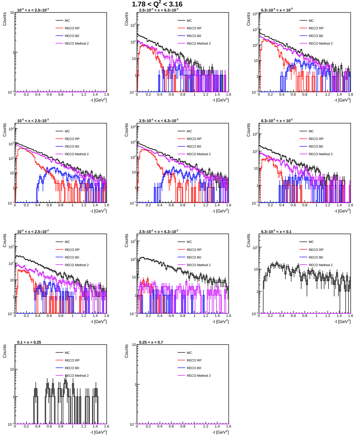
Figure 32: Comparison of the reconstructed -t distributions obtained using the Roman Pot (RP), B0, and Method 2 with the corresponding MC truth distribution for 1.78 < Q^2 < 3.16 \text{ GeV}^2 . Each panel represents a different Bjorken- x interval, illustrating the complementary detector acceptance and the contribution of Method 2 in recovering events within regions of reduced RP and B0 acceptance.
