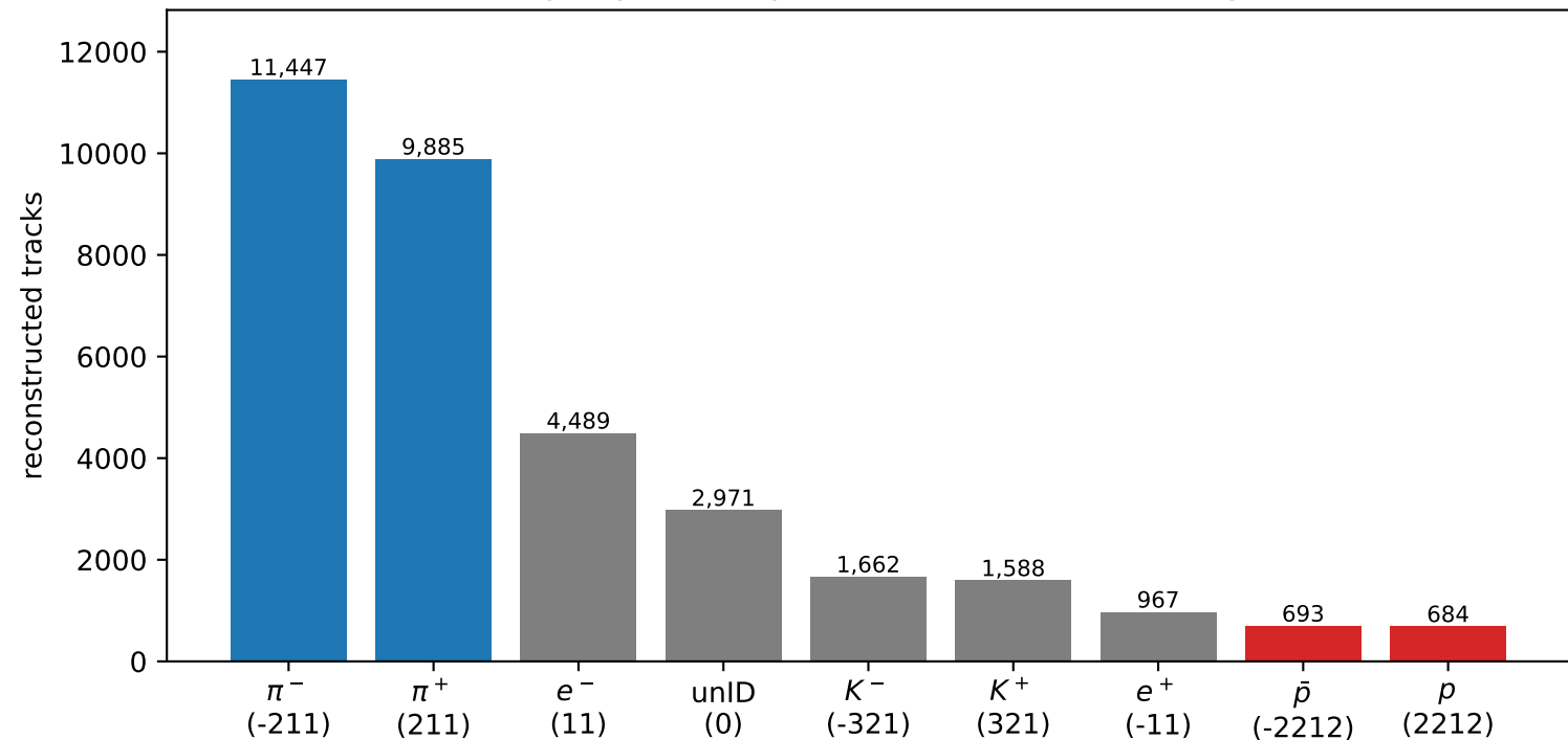
Reconstructed charged-particle species (ReconstructedChargedParticles.PDG)
