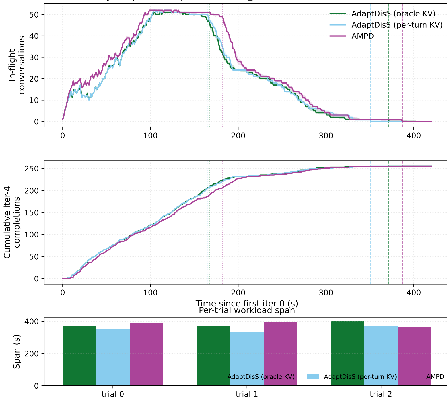
3-way comparison at rps=1.634, p300_d300 — 3 trials each (median + IQR)
