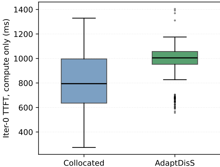
Iter-0 TTFT excl. network/queue (p300_d300 @ rps 1.634)
