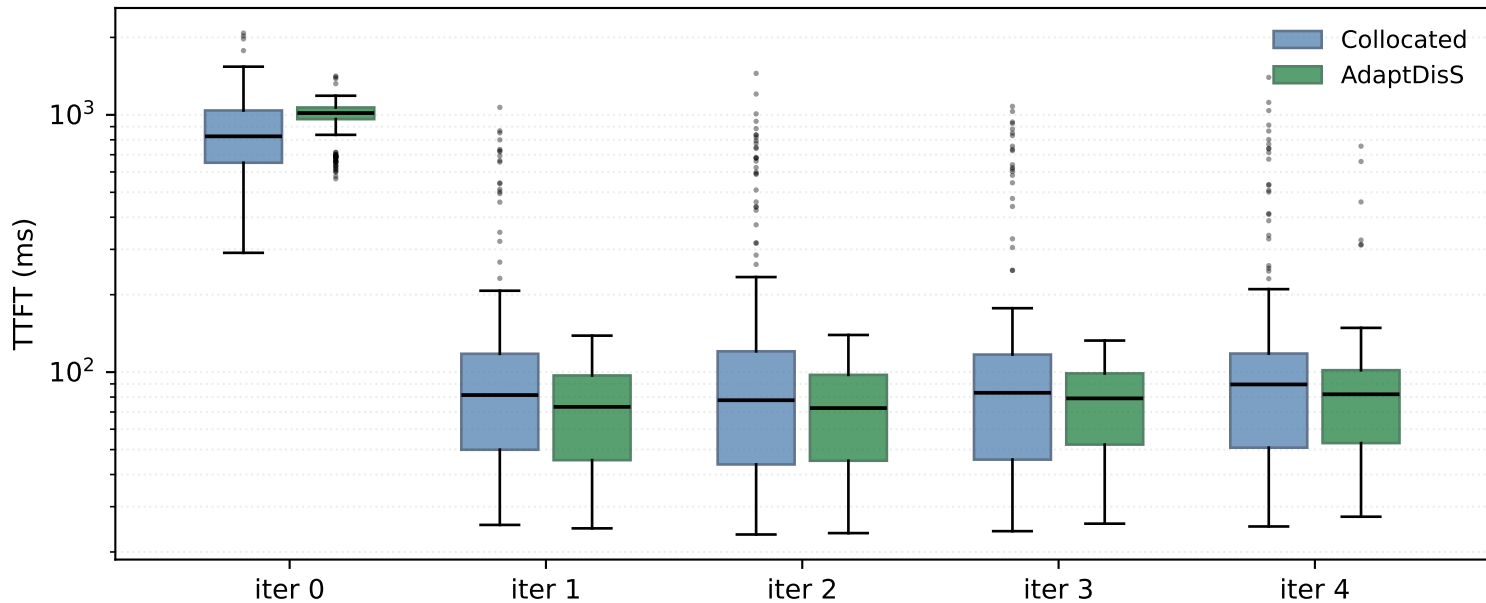
Per-turn TTFT, p300_d300 @ rps 1.634
