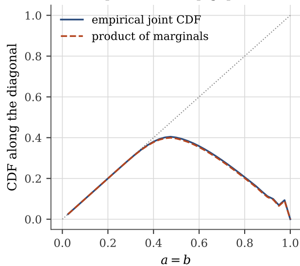
Independence: sup gap 0.005
