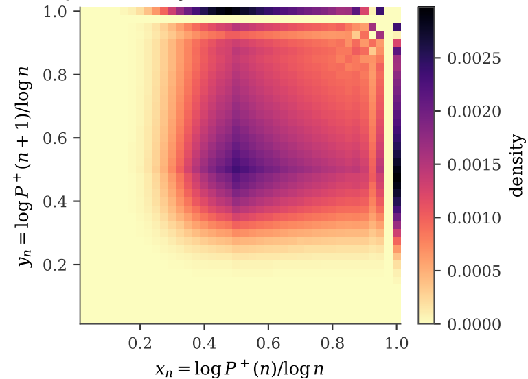
Joint density of the two coordinates
