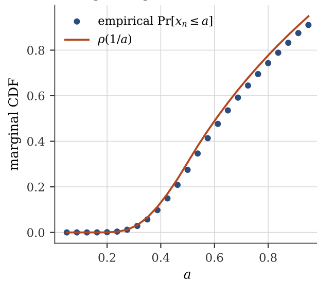
Marginal against the Dickman law
