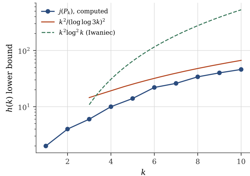
Jacobsthal values against the two bounds
