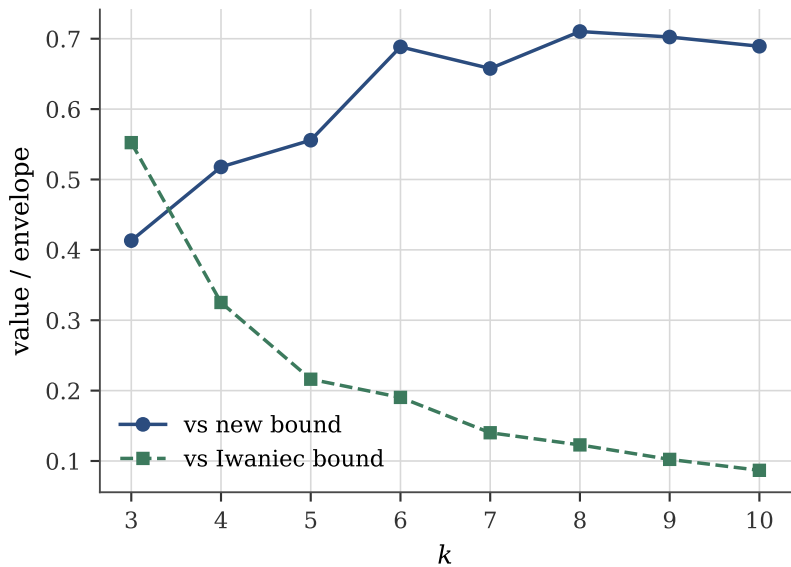
Implied constant in each bound
