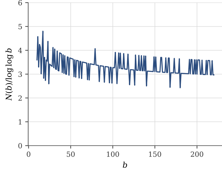
Empirical constant in the double-logarithmic order
