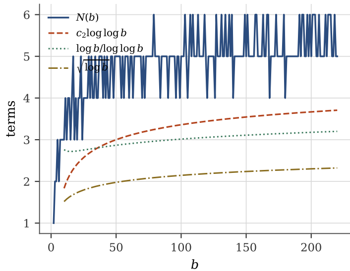
Growth against the bounds
