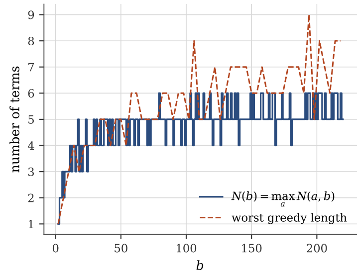
Minimum length against the greedy algorithm
