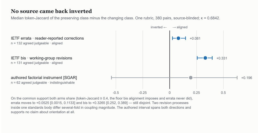
Figure 4: Lexical overlap differences between meaning-preserving and meaning-changing pairs under the uniform span construct rubric, per source, with bootstrap confidence intervals (§8).
