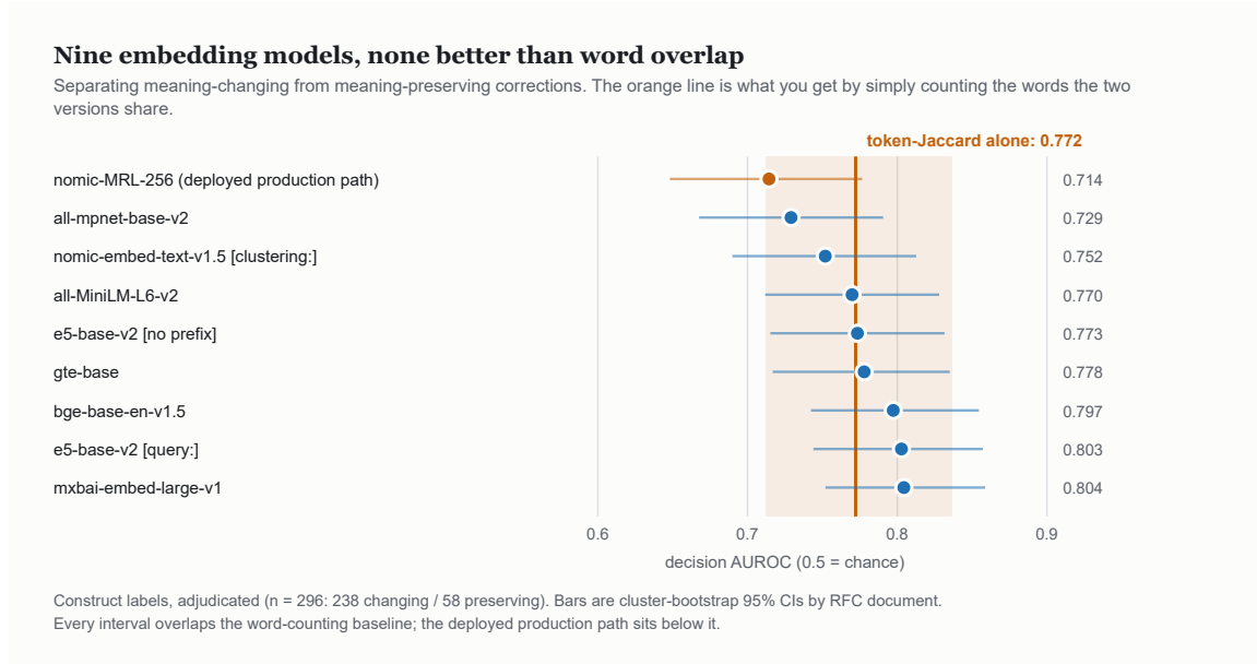
Figure 1: Encoder AUROC against the span-level construct labels on the adjudicated primary corpus, with the token-Jaccard word-counting baseline and the deployed production configuration marked (§4).
