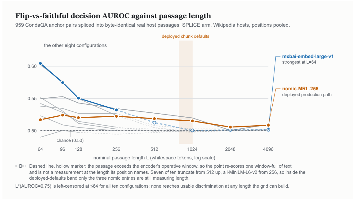
Figure 2: Decision AUROC, flip against faithful, against passage length, positions pooled, Wikipedia hosts. Dashed segments and hollow markers denote cells where the passage exceeds the encoder’s operative window (§5, Table 1).
