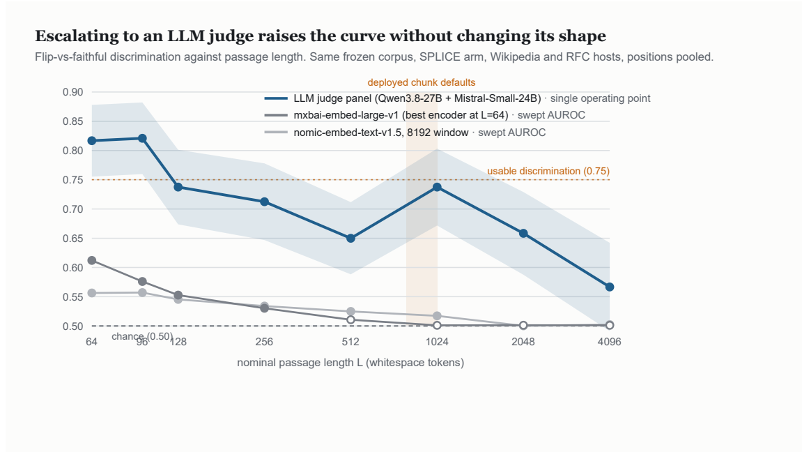
Figure 3: Flip against faithful discrimination against passage length for a language model judge panel and for two encoder configurations, on the same frozen corpus (SPLICE arm, Wikipedia and RFC hosts, positions pooled). The judge series is the area of a single-point ROC, (\text{TPR} + \text{TNR})/2 , over 120 mutation and 60 control judgments per length; the shaded band is its 95% confidence interval. Encoder series are swept AUROC from Table 1; hollow markers and dashed segments denote cells outside the encoder’s operative window. The judge sits well above every encoder and falls toward chance across the same range.
