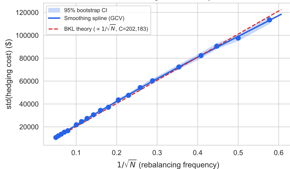
BKL variance scaling — FAIL: theory outside CI
