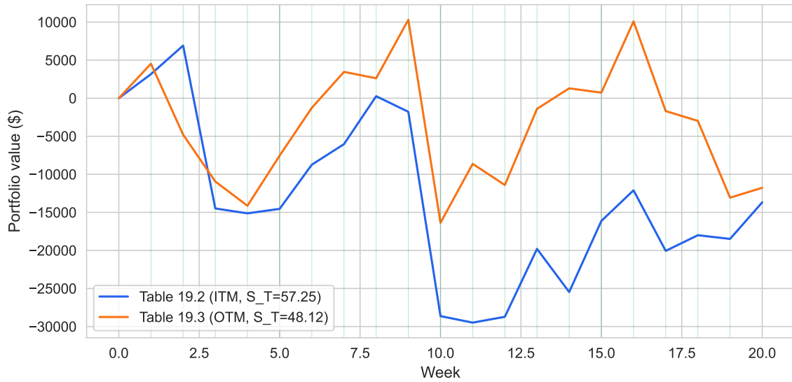
Figure 6.4: Portfolio value path for Hull Table 19.2 (ITM expiry, blue) and Table 19.3 (OTM expiry, orange). Green vertical lines mark step-certificate passes; no failures observed in either path. Source: Hull (2014) Tables 19.2–19.3.
